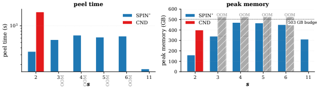
Figure 7: com-friendster (1.806B edges): peel time (left) and peak memory (right). CND completes only at s=2 ; on the tested cells with s \geq 3 , it exceeds the 503 GB budget.
