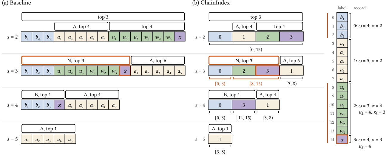
Figure 2: Baseline (a) and ChainIndex (b) for Figure 1, one row per size; tints mark chains, orange the query of x at (3, 2) .
