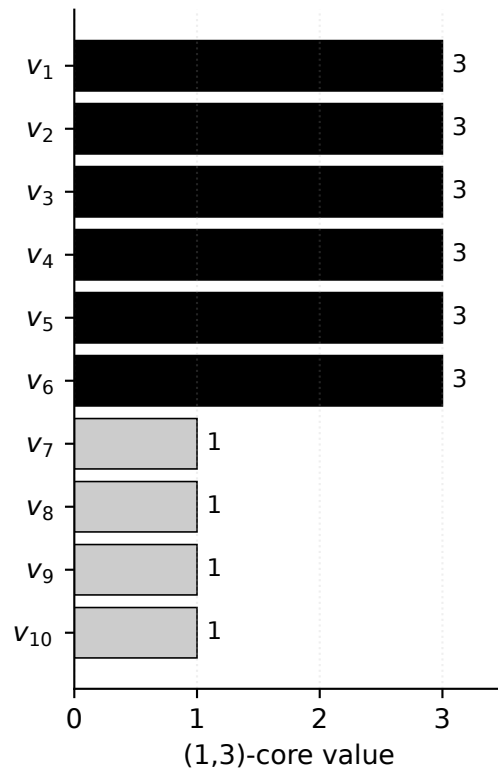
(c) Peeling output
