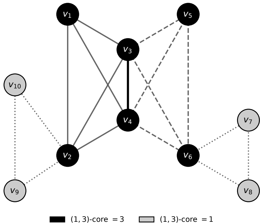
(a) Input graph G : |V| = 10 , |E| = 17 , 10 triangles at s = 3
