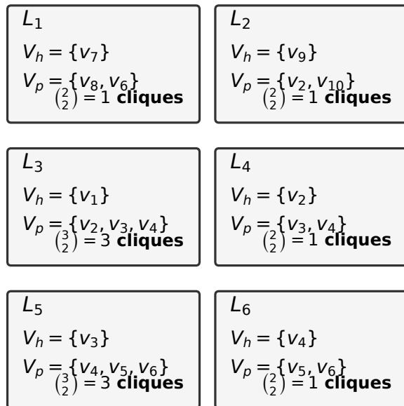
(b) Clique Path Index: 6 leaves encoding all 10 triangles
