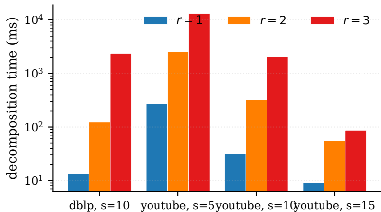
decomposition time (lower is better)
