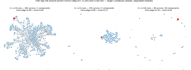
Figure 16: Two-hop ego-network of a com-dblp anchor under (1, s) -decomposition. Vertices are colored by connected component among surviving vertices. Observe that increasing s splits one large local structure into smaller components.
