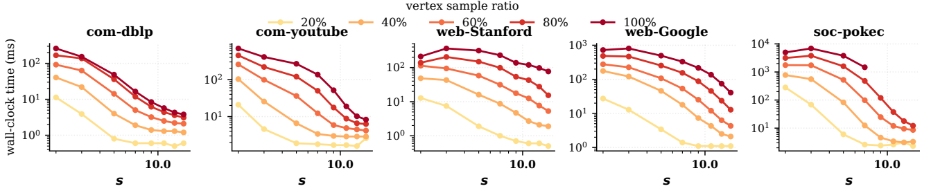
Figure 10: Vertex-induced scalability of SPIN*: wall-clock time as s varies on five graphs, one curve per vertex-sample ratio. Higher ratios consistently take longer; the curves do not cross.
