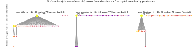
Figure 17: (1, s) -clique-connected nucleus join tree at s = 5 across three domains. Observe that the hierarchy shapes differ across collaboration, social, and web graphs.
