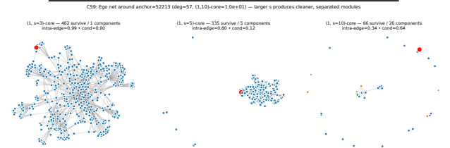
Figure 16: Two-hop ego-network of a com-dblp anchor under (1, s) -decomposition. Vertices are colored by connected component among surviving vertices. Observe that increasing s splits one large local structure into smaller components.
