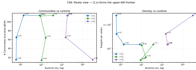
Figure 14: Quality-runtime Pareto plot on com-dblp for r \in \{1, 2, 3\} and s \in \{5, 10, 15, 20\} . Observe that the r = 1 points lie on the favorable quality-runtime frontier in the DBLP settings.
