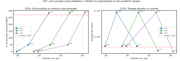
Figure 12: Quality-runtime Pareto plot on com-youtube for r \in \{1, 2, 3\} and s \in \{5, 10, 15\} . Observe that r = 1 reaches the same quality contours as higher- r settings with lower runtime.
