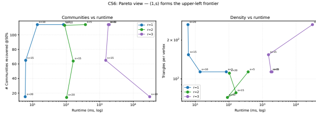
Figure 11: Quality-runtime Pareto plot on com-dblp for r \in \{1, 2, 3\} and s \in \{5, 10, 15, 20\} . Observe that the r = 1 points lie on the favorable quality-runtime frontier in the DBLP settings.
