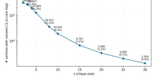
Figure 9: Active-set size on com-dblp as s varies. Observe that larger s sharply shrinks the vertices with nonzero (1, s) -core value.
