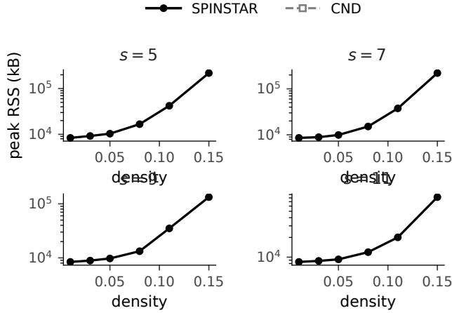
Figure 8: Peak resident-set memory under the same stress-test protocol as Figure 7. The memory gap shows when mutable residual state amplifies dense-clique growth.
