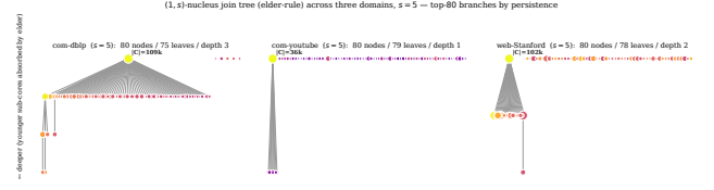
Figure 16: (1, s) -clique-connected nucleus join tree at s = 5 across three domains. Observe that the hierarchy shapes differ across collaboration, social, and web graphs.
