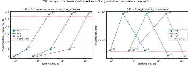
Figure 14: Quality-runtime Pareto plot on com-youtube for r \in \{1, 2, 3\} and s \in \{5, 10, 15\} . Observe that r = 1 reaches the same quality contours as higher- r settings with lower runtime.
