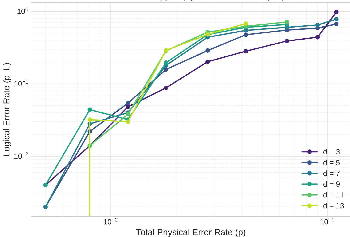
Surface Code Threshold Biased Noise ( \eta=10 ) | Meas Ratio: 10 (3D)
