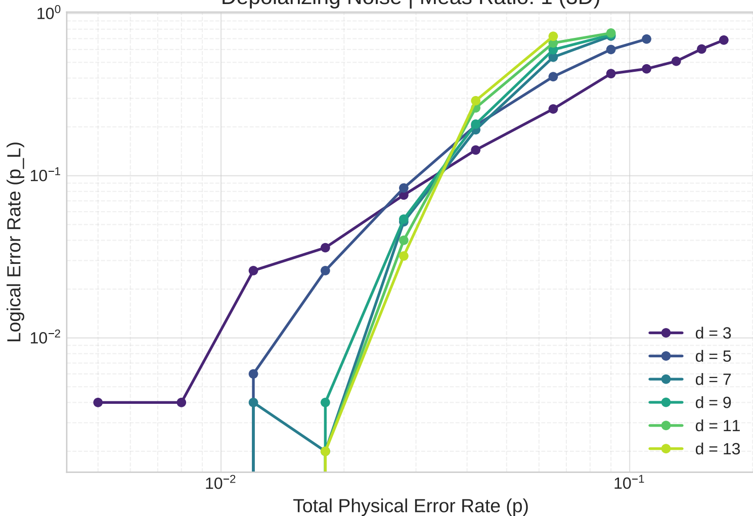
Surface Code Threshold Depolarizing Noise | Meas Ratio: 1 (3D)
