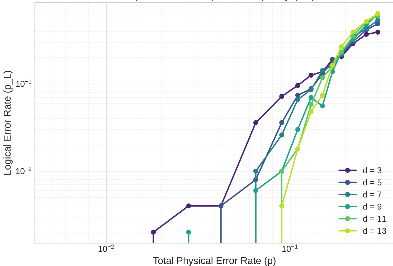
Surface Code Threshold Independent Noise | Code Capacity (2D)
