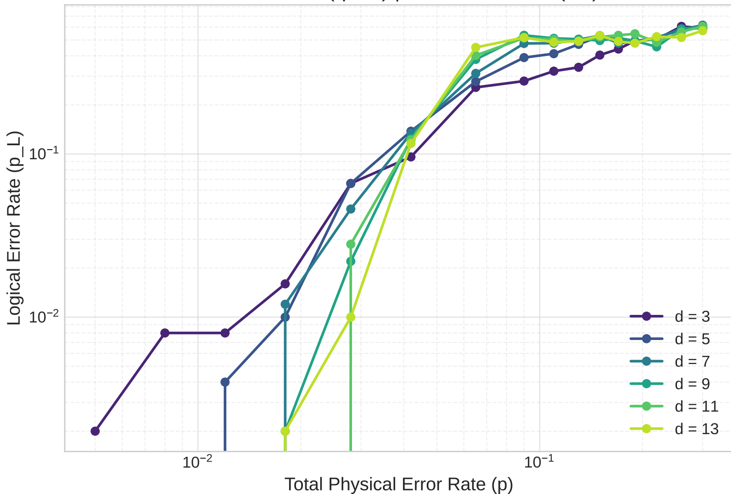
Surface Code Threshold Biased Noise ( \eta=10 ) | Meas Ratio: 0.1 (3D)
