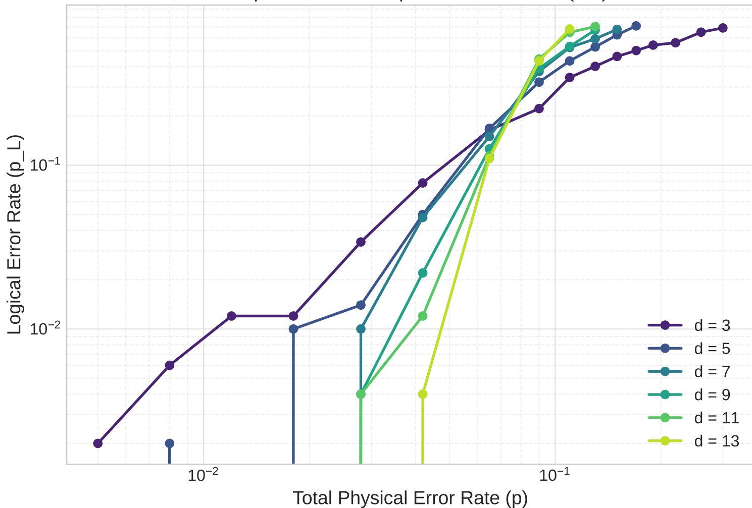
Surface Code Threshold Independent Noise | Meas Ratio: 0.1 (3D)
