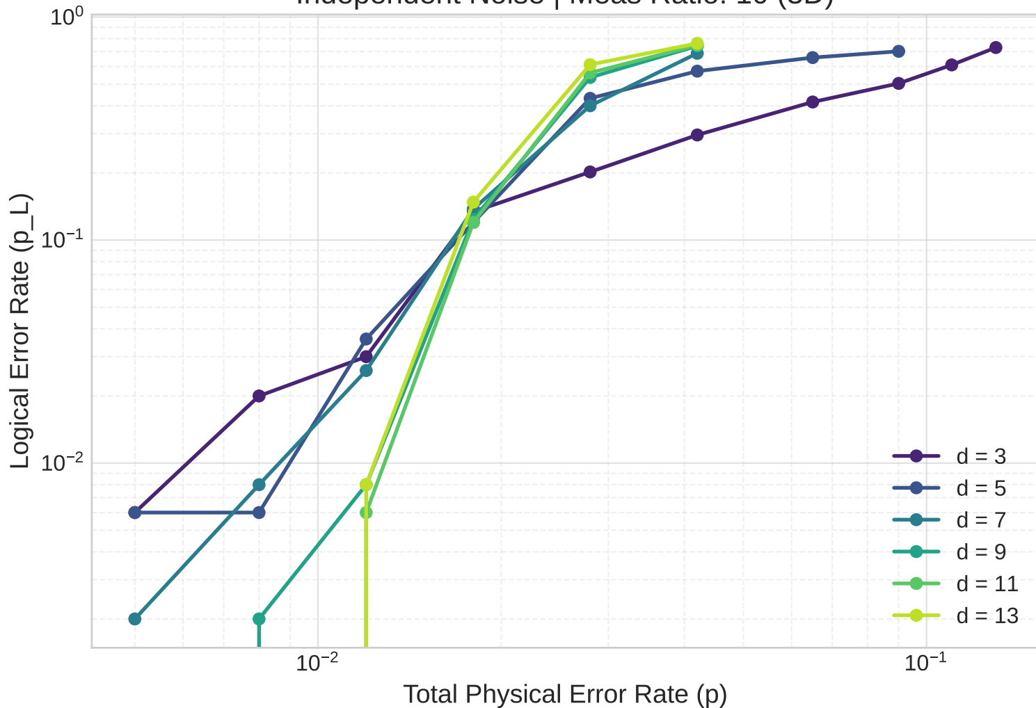
Surface Code Threshold Independent Noise | Meas Ratio: 10 (3D)
