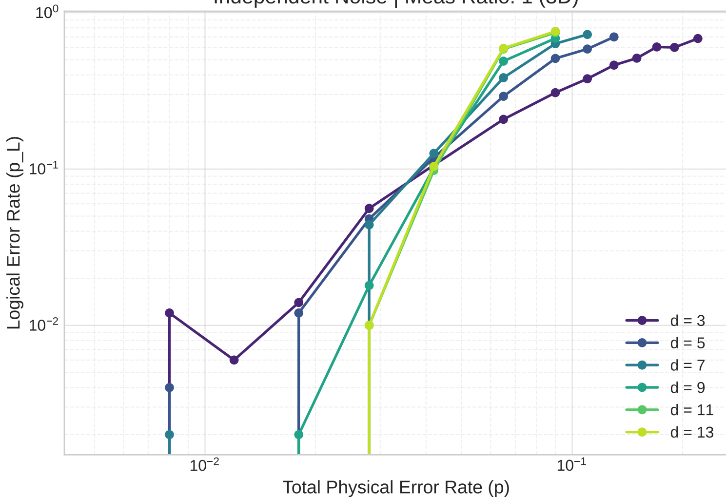
Surface Code Threshold Independent Noise | Meas Ratio: 1 (3D)
