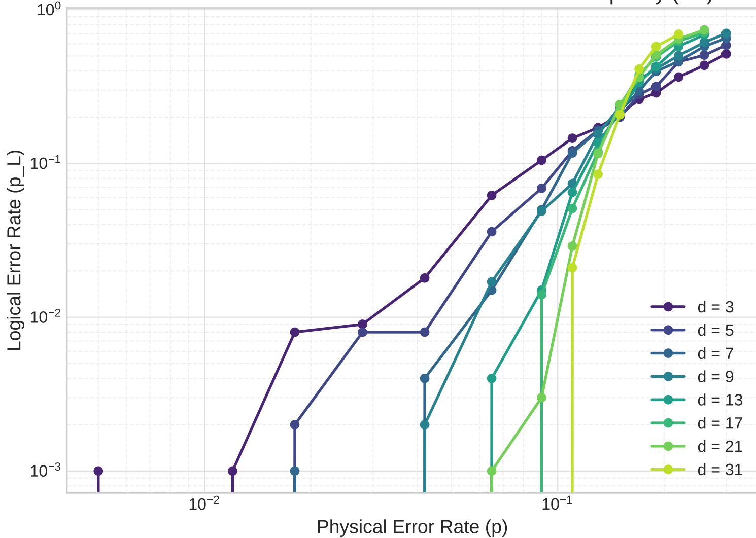
Surface Code Error Correction Threshold - Code Capacity (2D)
