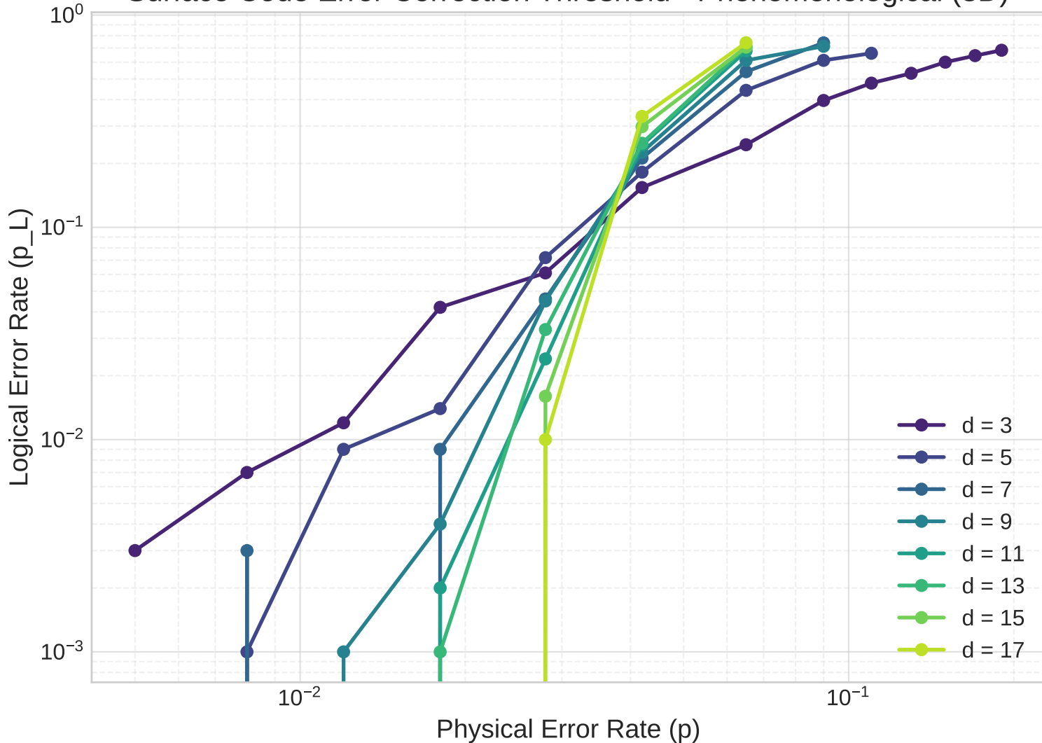
Surface Code Error Correction Threshold - Phenomenological (3D)
