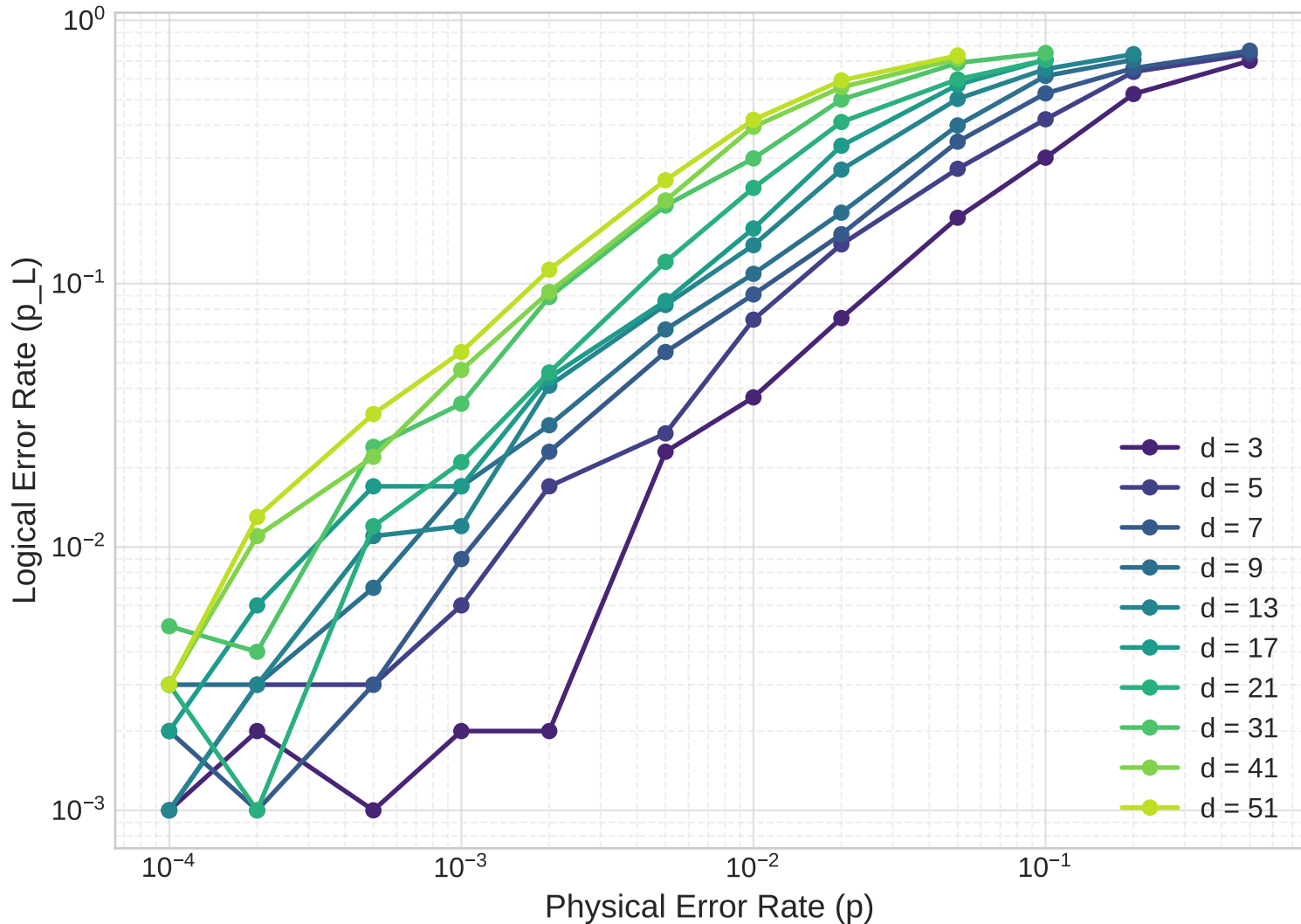
Surface Code Error Correction Threshold
