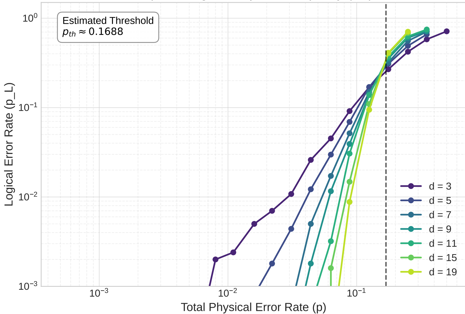
Surface Code Threshold Depolarizing Noise | Code Capacity (2D)
