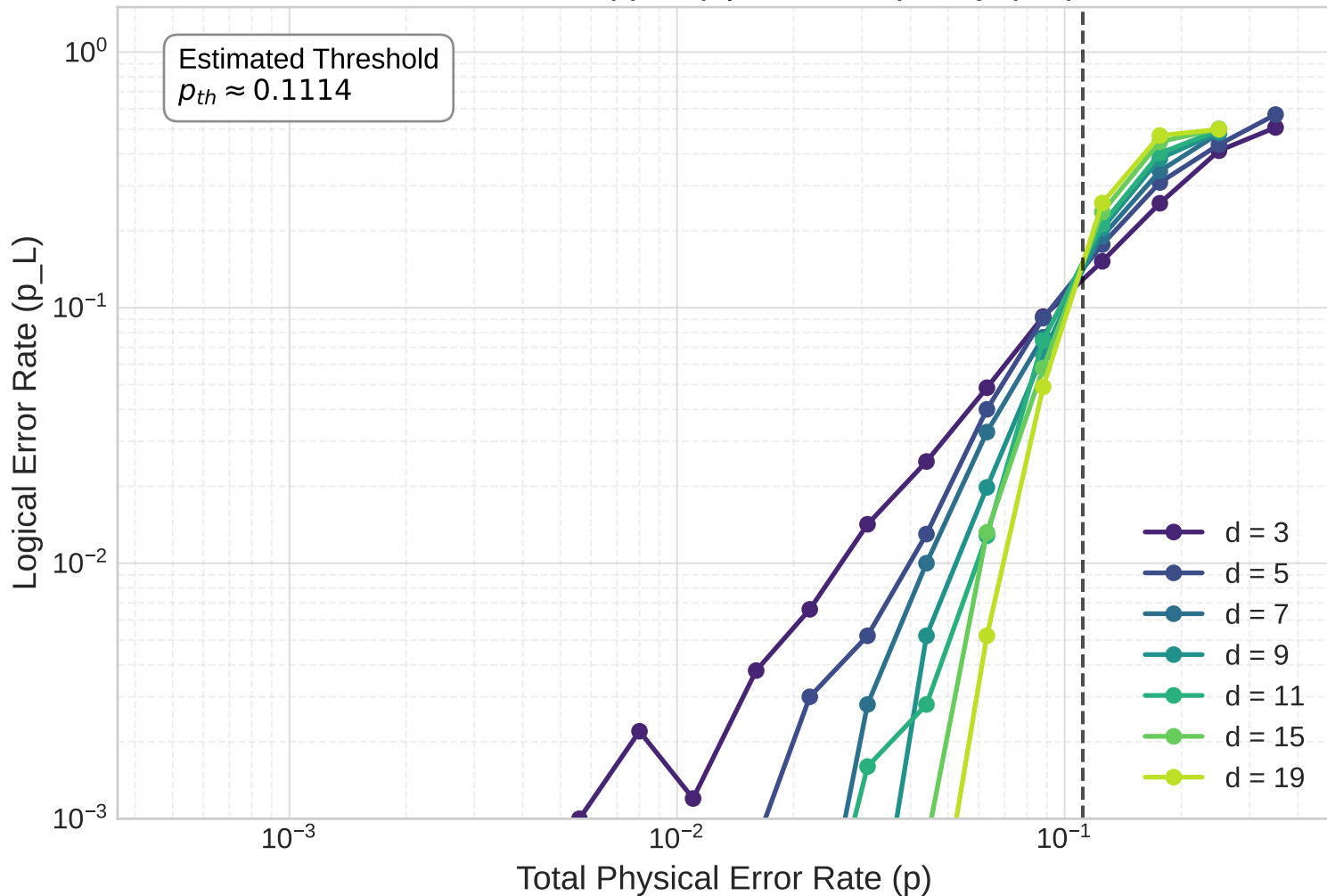
Surface Code Threshold Biased Noise ( \eta=10 ) | Code Capacity (2D)
