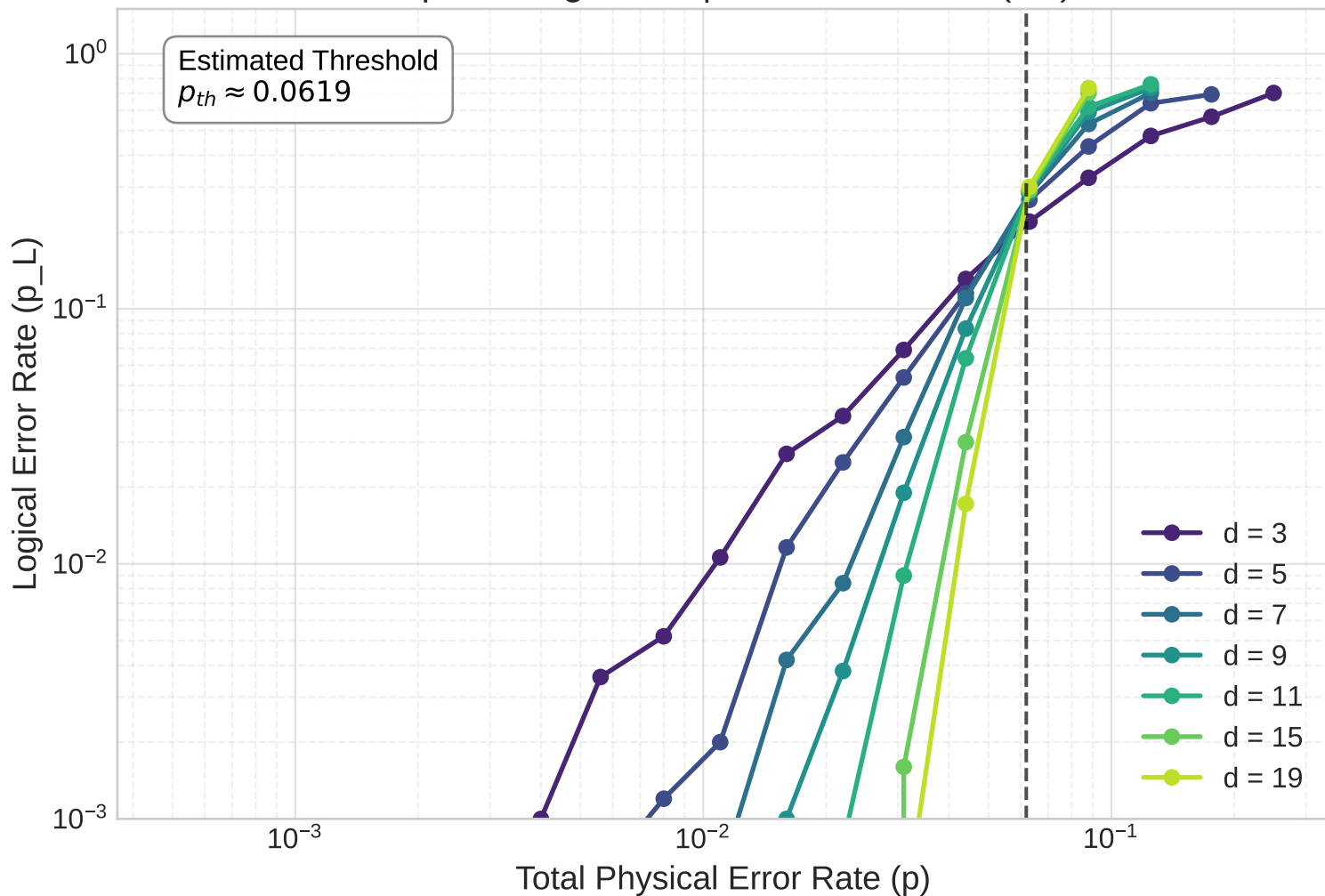
Surface Code Threshold Depolarizing Noise | Meas Ratio: 0.1 (3D)
