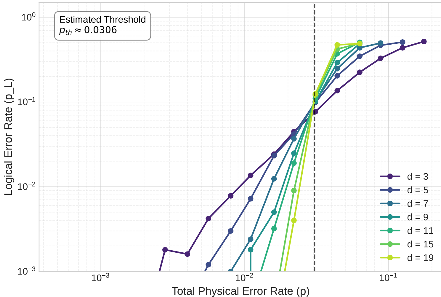
Surface Code Threshold Biased Noise ( \eta=10 ) | Meas Ratio: 1 (3D)
