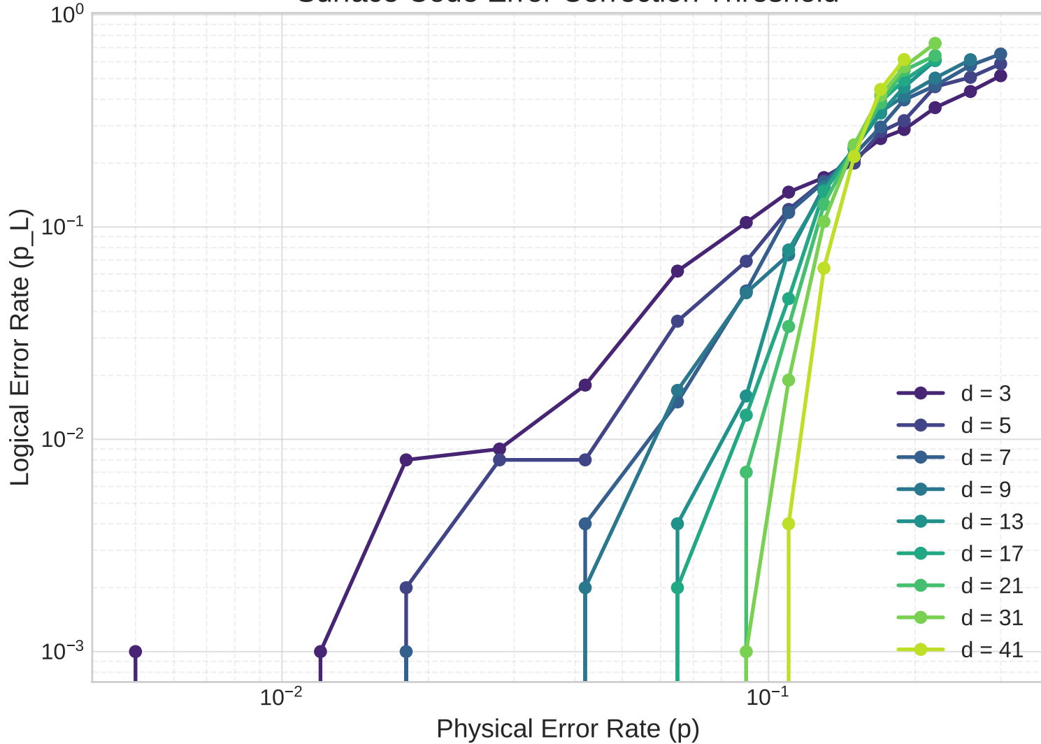
Surface Code Error Correction Threshold
