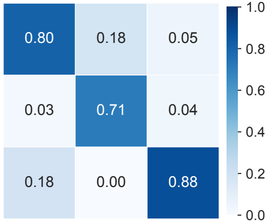
Cosine similarity
