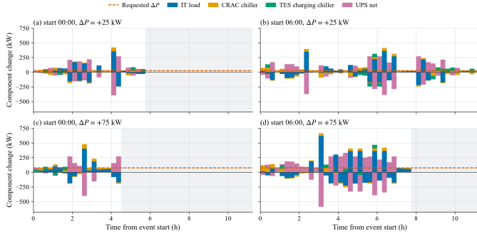
Fig. 9. DC component contributions to downward flexibility (positive \Delta P ). Rows correspond to the requested flexibility magnitudes (+25 and +75 kW, top to bottom) and columns to the start times (00:00, left; 06:00, right). Colours show the flexibility contribution of each DC asset.
