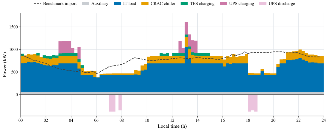
Fig. 6. Optimised DC Component Power Consumption
