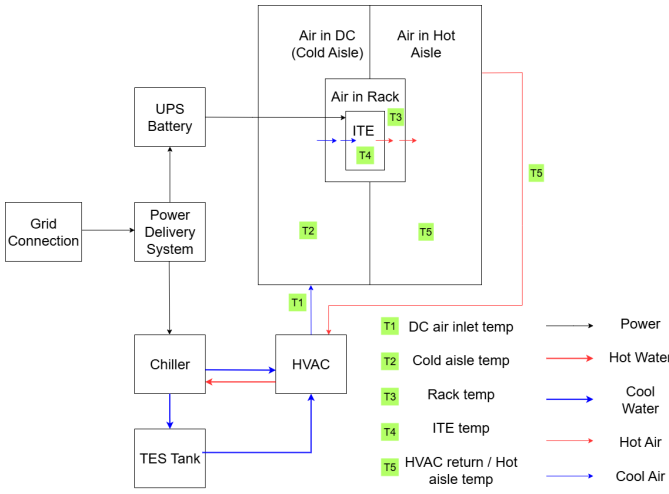
Fig. 1. Data Centre Layout
