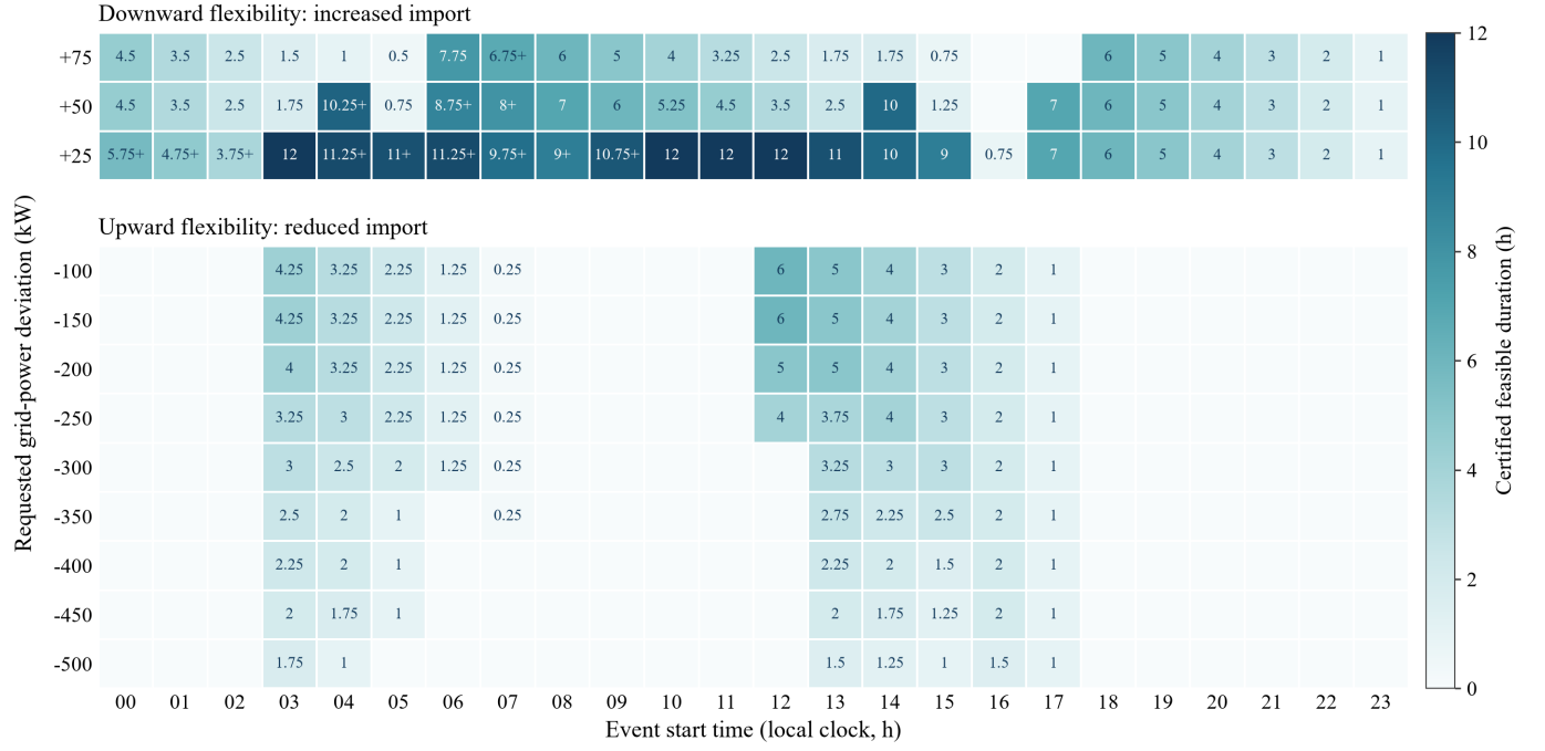
Fig. 7. Flexibility provision magnitude and duration. Cell values are certified feasible durations \tau in hours for each start time t_0 (x-axis) and requested power deviation \Delta P (y-axis). Positive \Delta P (top three rows) denotes downward flexibility (load increase) and negative \Delta P denotes upward flexibility (load reduction). A plus sign marks an unresolved next 15-minute trial. Blank cells have no positive duration certified by the search; twelve-hour and local-day-end values are assessment-capped.
