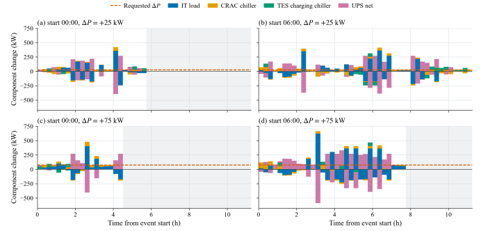
Fig. 9. DC component contributions to downward flexibility (positive \Delta P ). Rows correspond to the requested flexibility magnitudes ( +25 and +75 kW, top to bottom) and columns to the start times (00:00, left; 06:00, right). Colours show the flexibility contribution of each DC asset.
