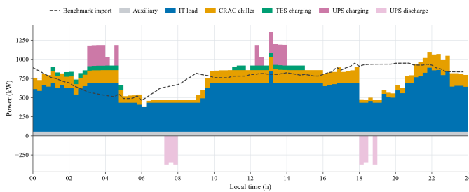
Fig. 6. Optimised DC Component Power Consumption
