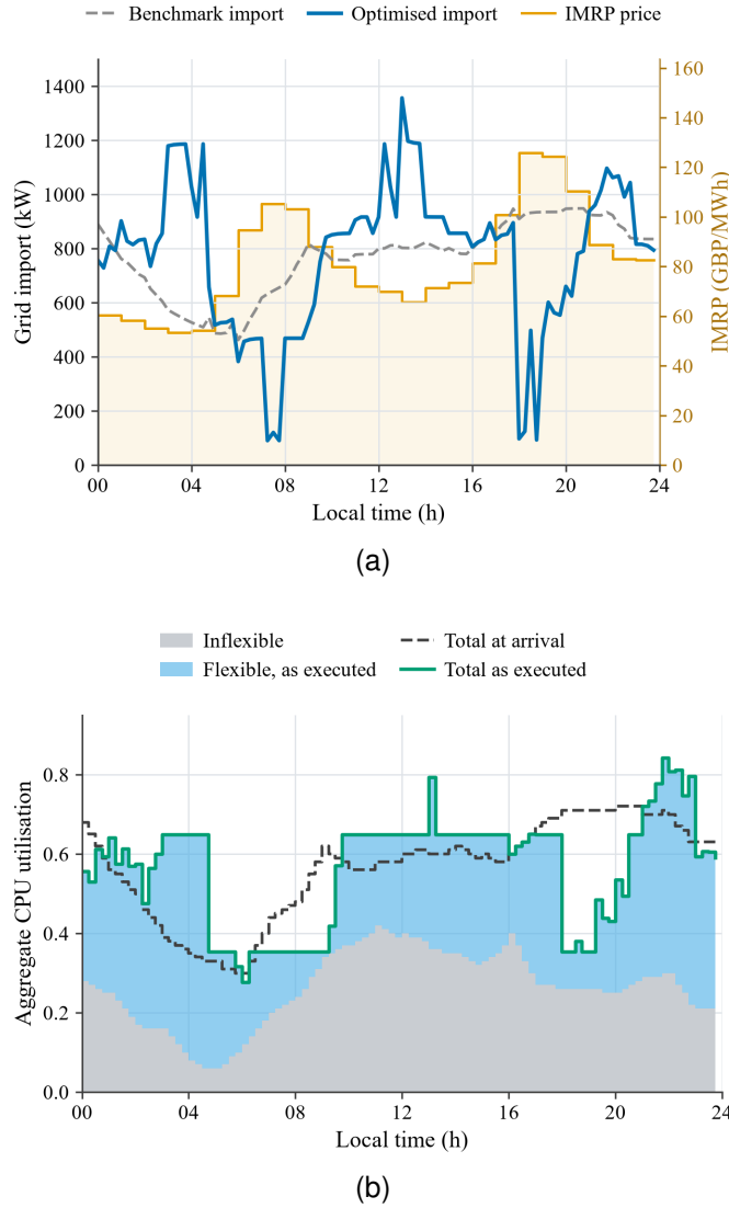
Fig. 5. (a) Grid power and reference prices on 22 September 2025. (b) The corresponding IT workload arrival and execution profiles. Scenario 2 supplies the undisturbed trajectory for the event assessment.
