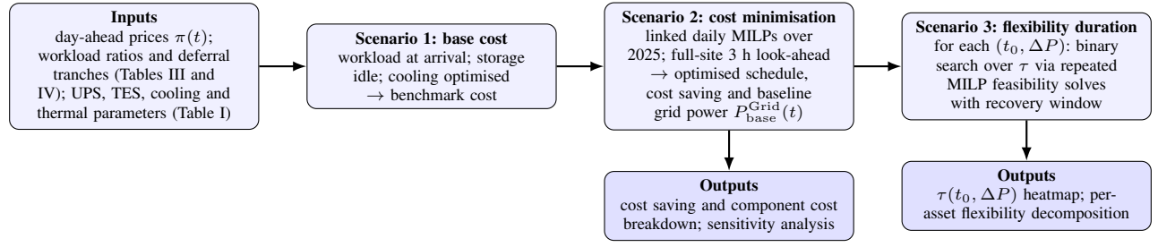
Fig. 4. Workflow of the three-scenario optimisation and flexibility assessment. Scenario 1 provides the workload-at-arrival cost benchmark, Scenario 2 establishes the cost-optimised baseline, and Scenario 3 identifies certified feasible flexibility durations for each requested start time and power deviation while enforcing recovery.
