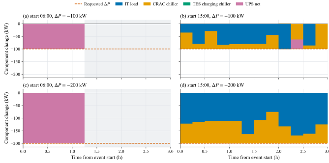
Fig. 8. DC component contributions to upward flexibility (negative \Delta P ). The four panels are arranged in a 2-by-2 grid: rows correspond to the requested flexibility magnitudes ( -100 and -200 kW, top to bottom) and columns to the start times (06:00, left; 15:00, right). Colours show the flexibility contribution of each DC asset.
