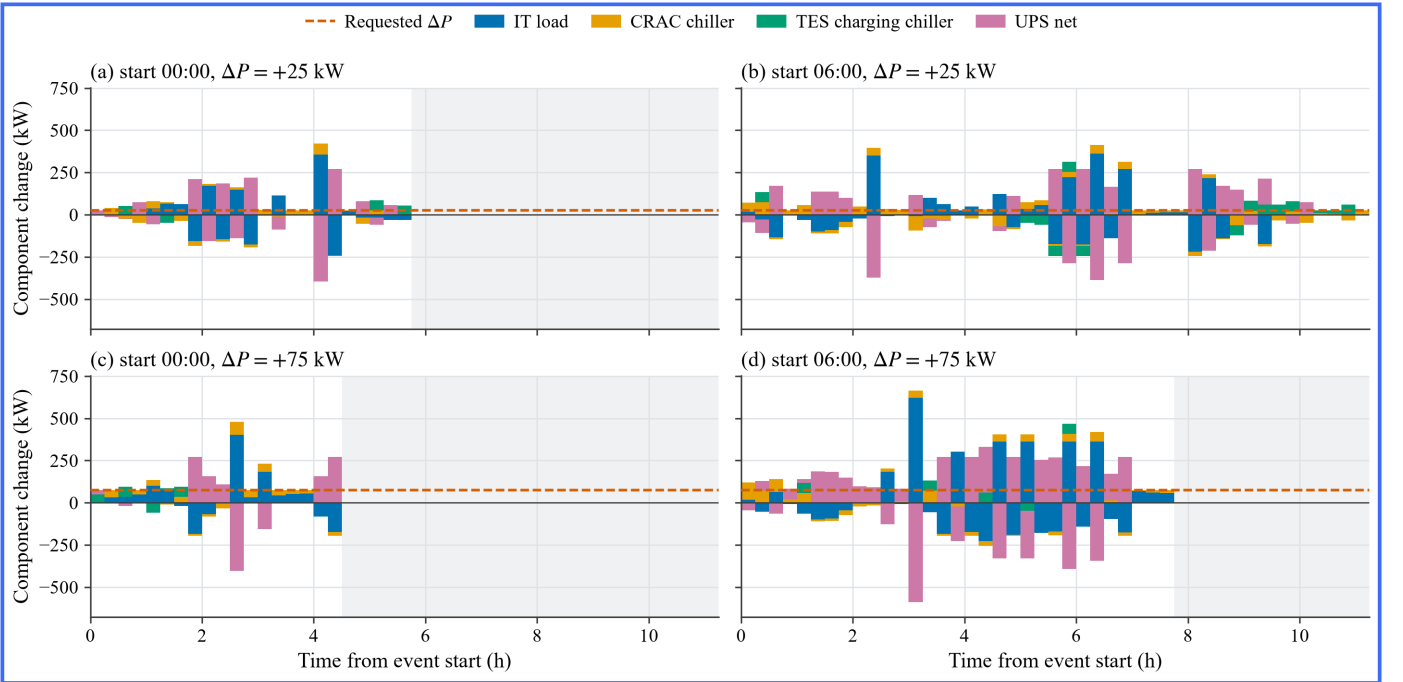
Fig. 9. Component decomposition for selected increased import events. Notation is as in Fig. 8.
