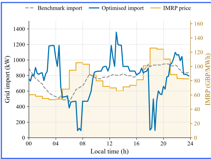
(a) Grid import and IMRP price.
