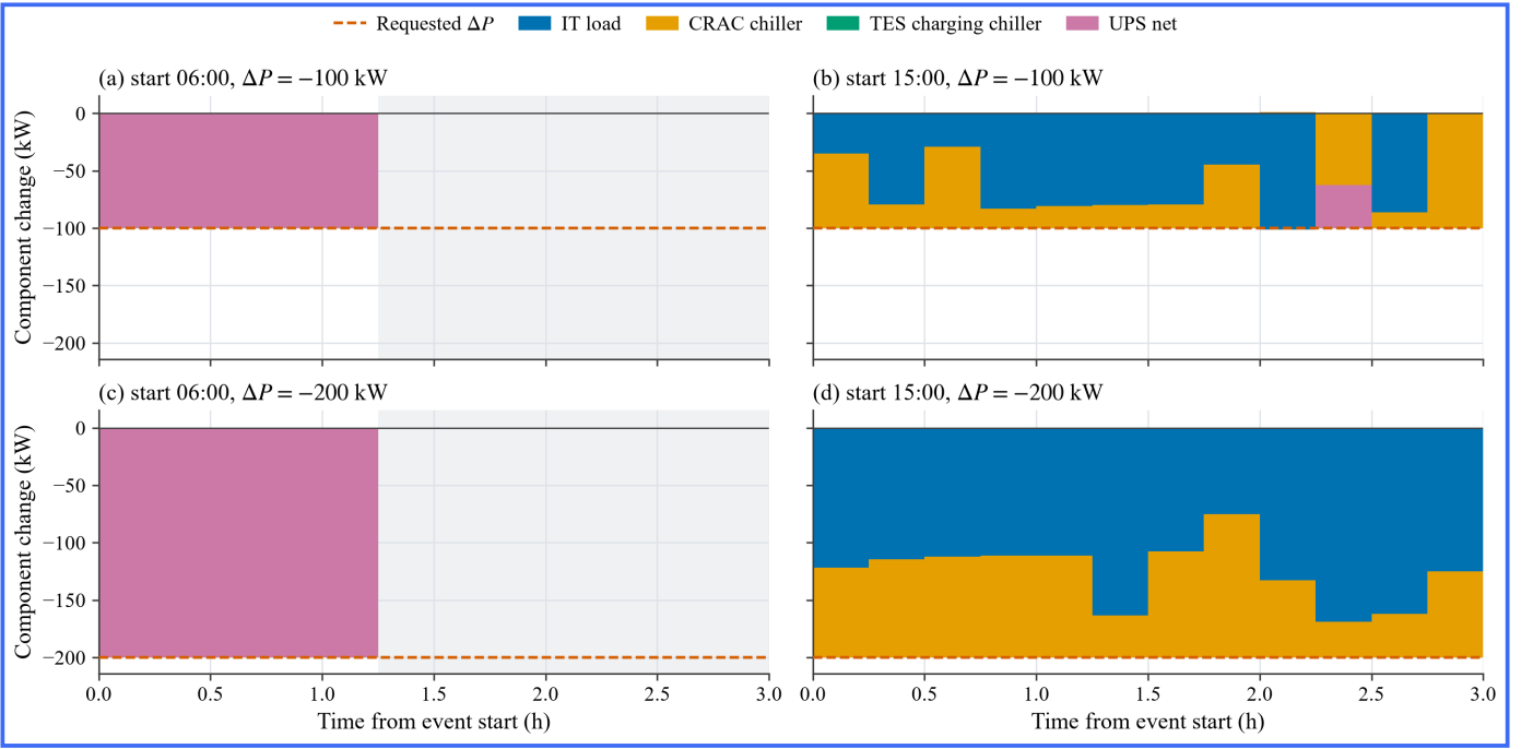
Fig. 8. Component decomposition for selected reduced import events. Positive and negative component changes are stacked separately and sum to the dashed requested deviation. The grey area begins after the certified event duration.
