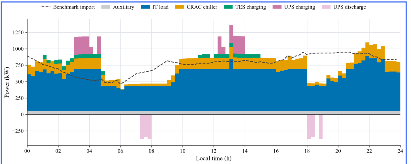
Fig. 6. Optimised component dispatch on 22 September 2025. Bars above the axis are metered demand. UPS discharge appears below the axis because it supplies IT demand behind the meter. The dashed line is benchmark grid import.
