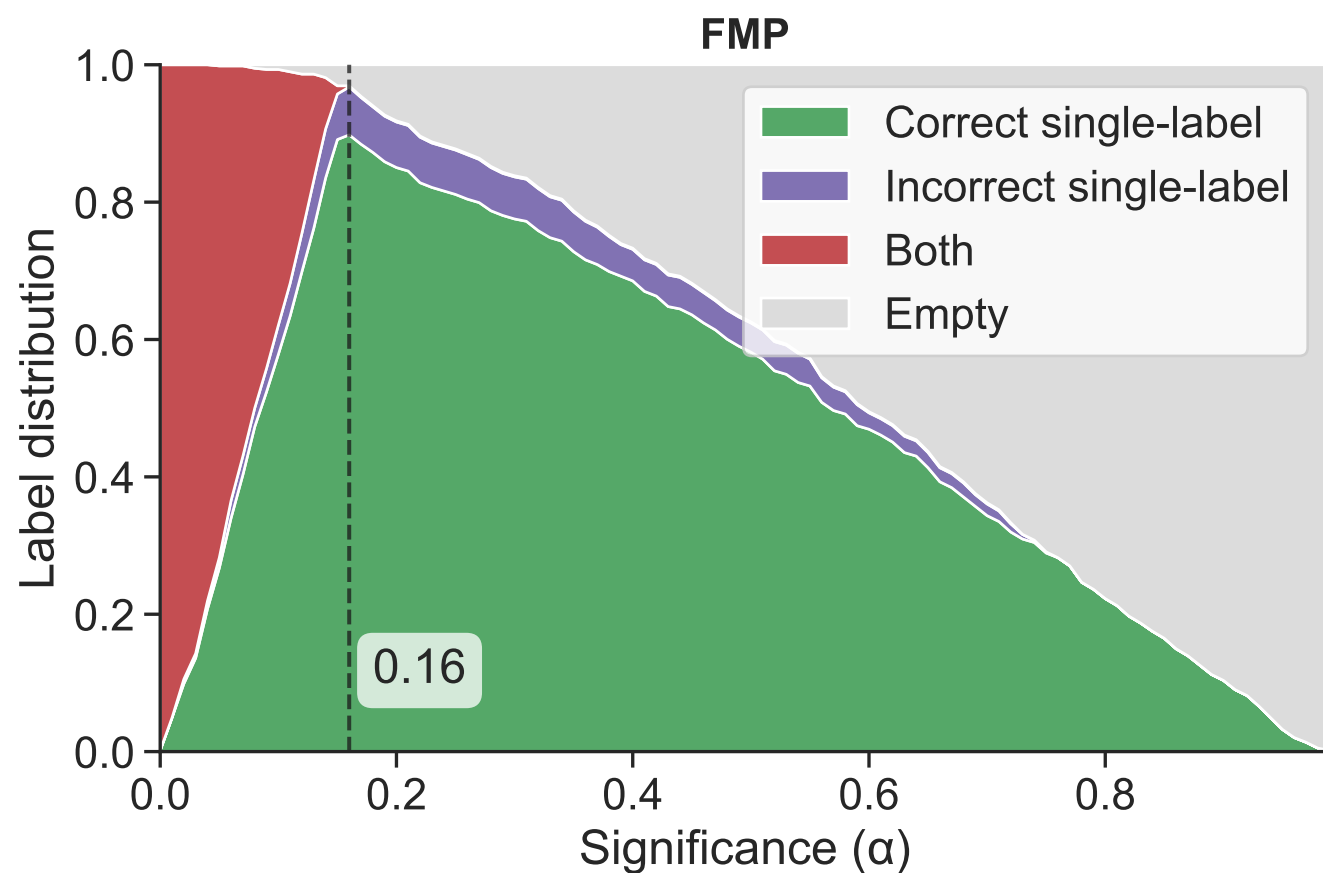
(a) Label Distribution
