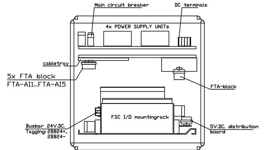
FRONT CROSS SECTION-AA
