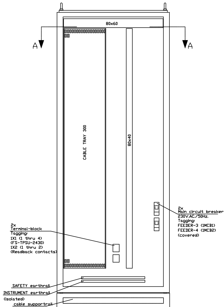
FRONT VIEW WITHOUT SWINGFRAME
