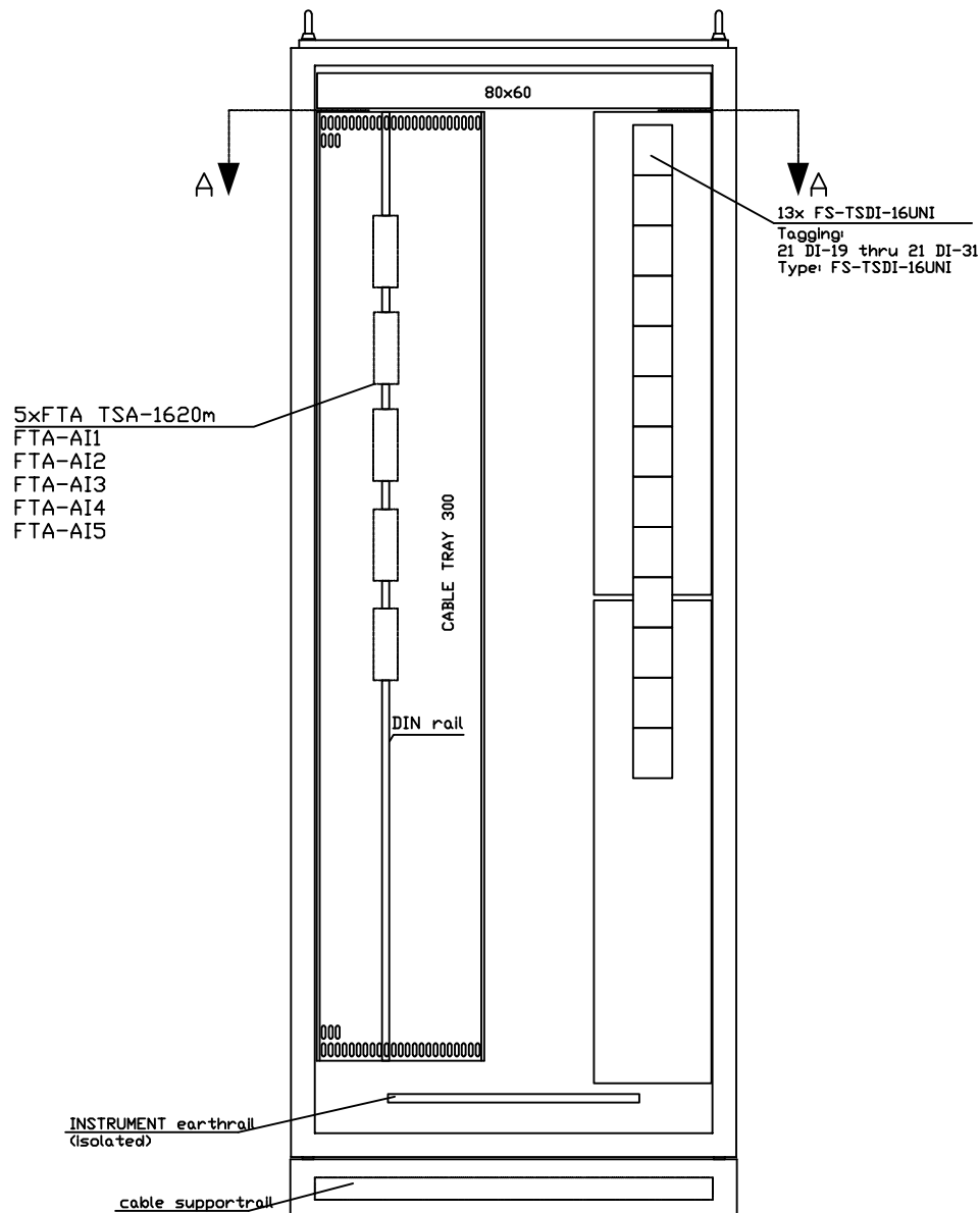
FRONT VIEW WITHOUT SWINGFRAME
