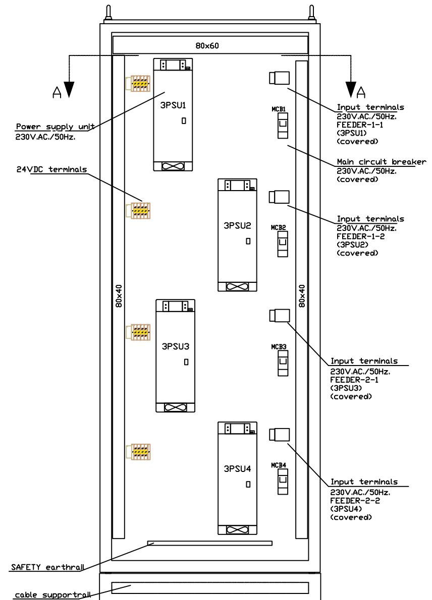
REAR VIEW WITHOUT DOOR(S)
