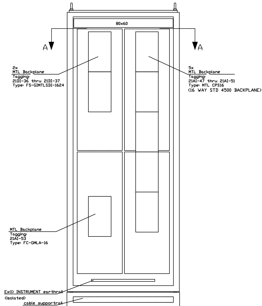
REAR VIEW WITHOUT DOOR(S)
