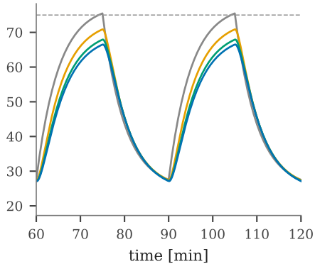
thermostat duty (last 2 cycles)
