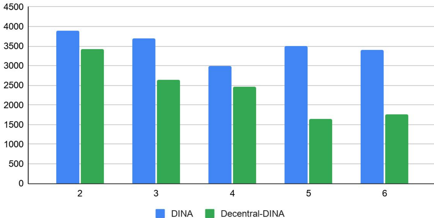
TPC-H query workload execution time in second (1,100 queries), by number of nodes, using TPC-H sf 10 database
