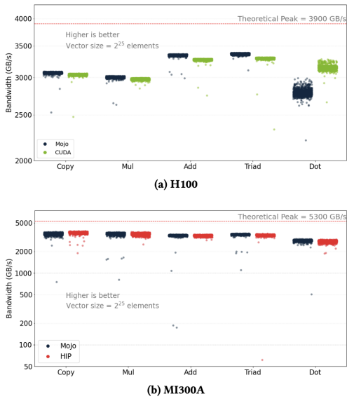
Figure 11: Mojo vs CUDA and HIP performance for BabelStream kernels on the NVIDIA H100 and AMD MI300A [9].
