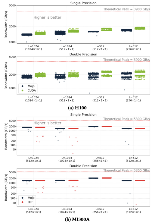
Figure 10: Mojo vs CUDA and HIP performance for the seven-point stencil kernel on the NVIDIA H100 and AMD MI300A [9].
