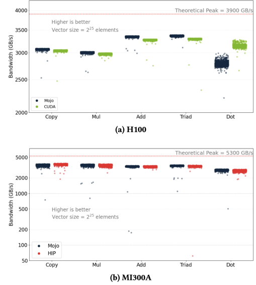
Figure 11: Mojo vs CUDA and HIP performance for BabelStream kernels on the NVIDIA H100 and AMD MI300A [9].
