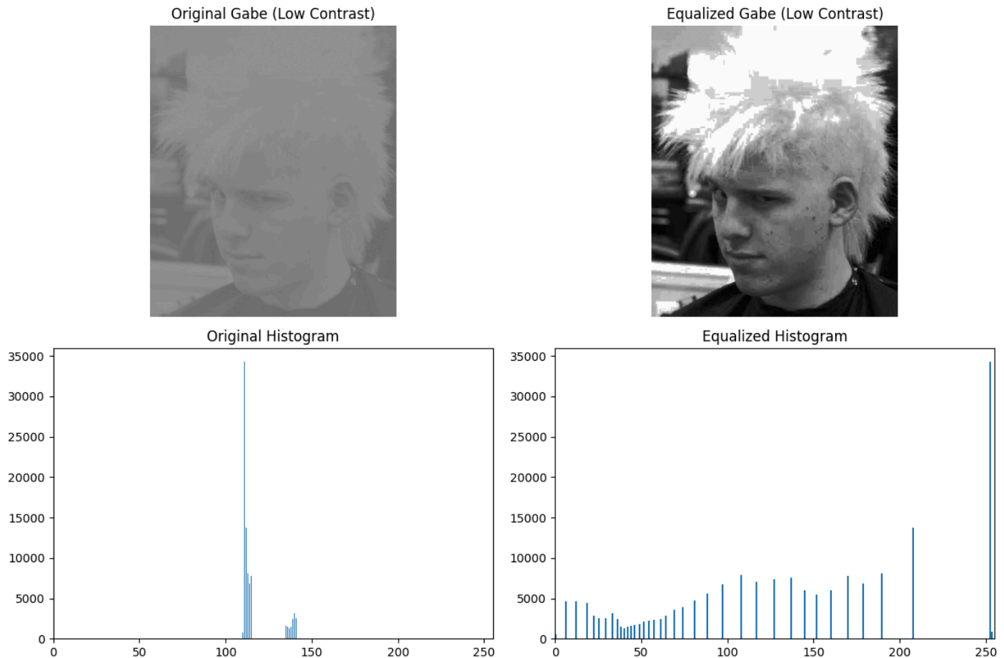
Figure 19: Comparison between the original low contrast image of Gabe and the histogram equalized image.
