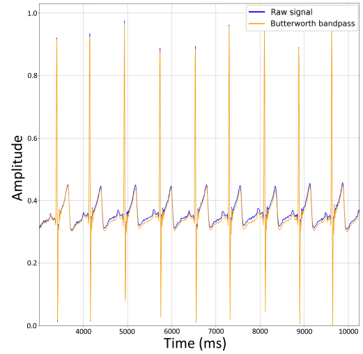
Figure 2: A comparison between raw and filtered ECG signals
