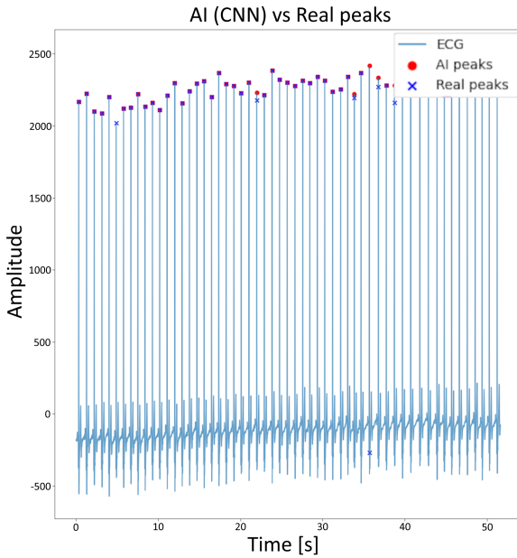
Figure 7: Comparison of R peak detection between the network and reference peaks
