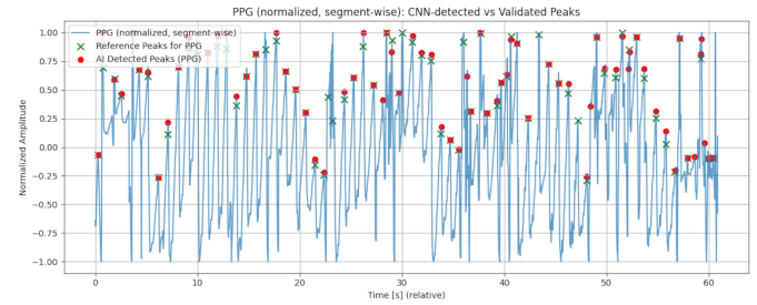
Figure 8: Peak detection comparison between the convolutional network and reference peaks
