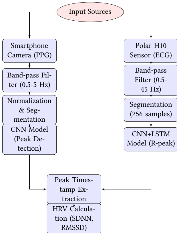
Figure 1: Block diagram of the proposed HRV analysis pipeline. The system processes ECG and PPG signals in parallel streams, applying specific filtering and deep learning models to extract peak timings for final HRV metric calculation.
