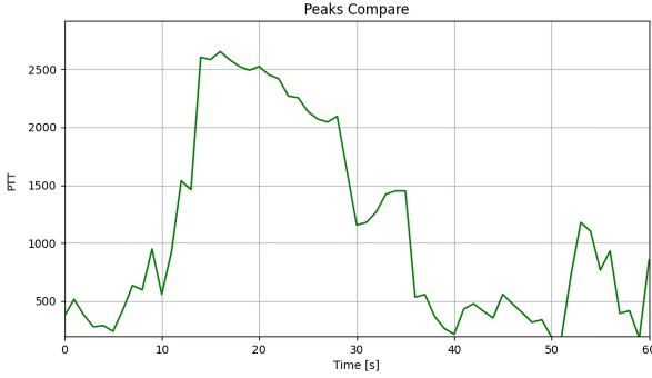
Figure 4: Time differences between ECG and PPG peaks
