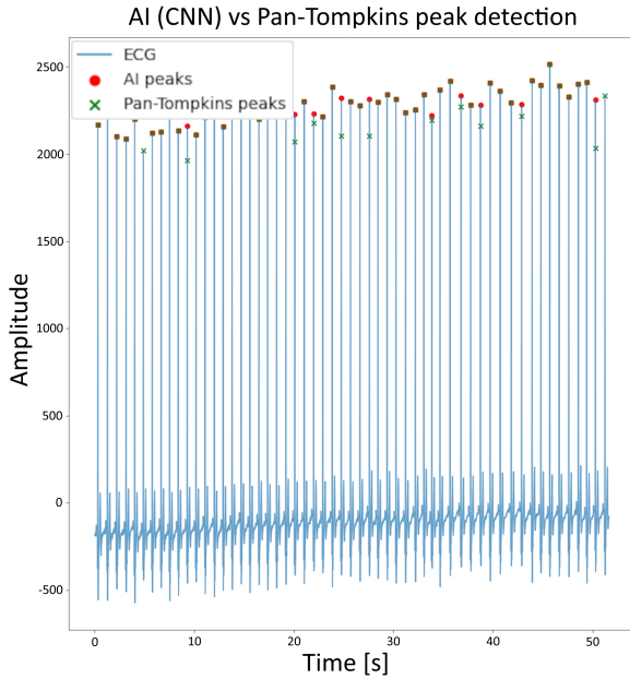
Figure 6: Comparison of R peak detection between the network and Pan-Tompkins algorithm
