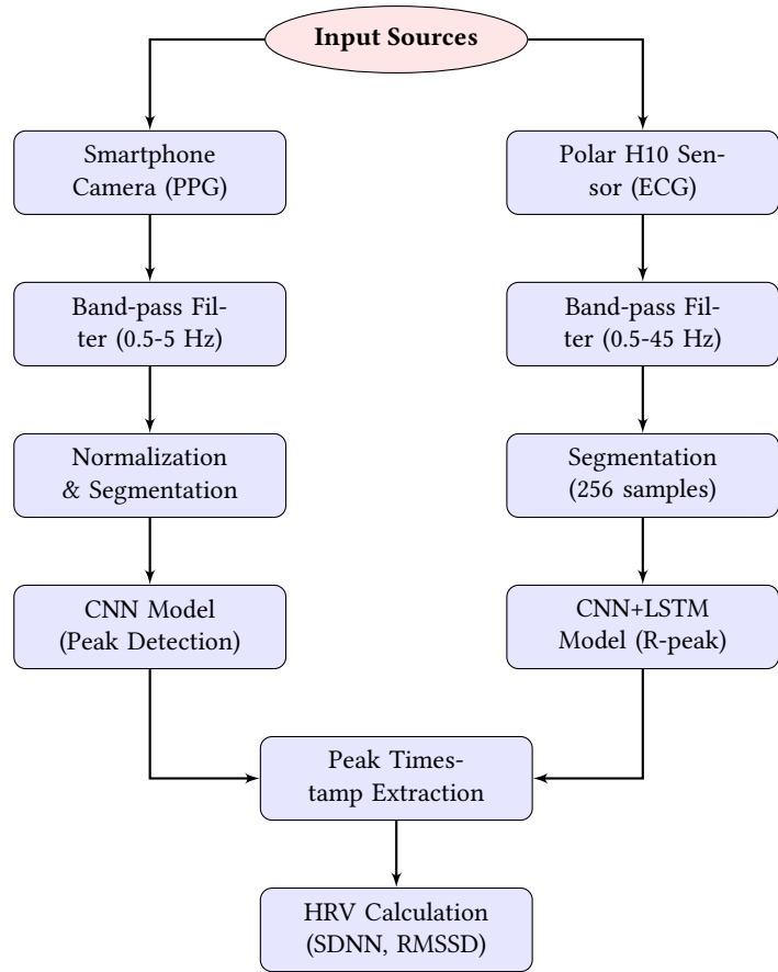
Figure 1: Block diagram of the proposed HRV analysis pipeline. The system processes ECG and PPG signals in parallel streams, applying specific filtering and deep learning models to extract peak timings for final HRV metric calculation.
