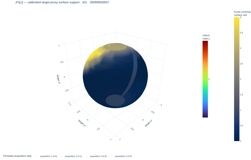
Figure 9: Calibrated selected-frustum support on the target-centred proxy sphere. The surface heat map is the complete equal-solid-angle coverage field; overlaid incidence samples preserve rollout and time heritage. This is not measured target-mesh visibility.
