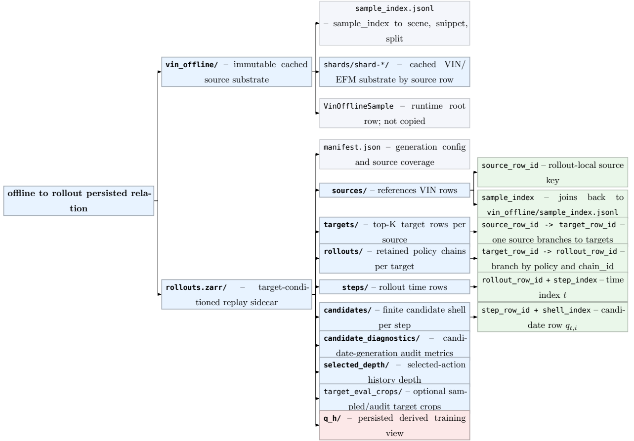
Figure 9: Relation between immutable VIN rows and target-conditioned replay. rollouts.zarr/ stores joins, target tasks, retained chains, full per-step candidate shells, selected-depth successor history, and a derived Q_H view without rewriting the source store.
