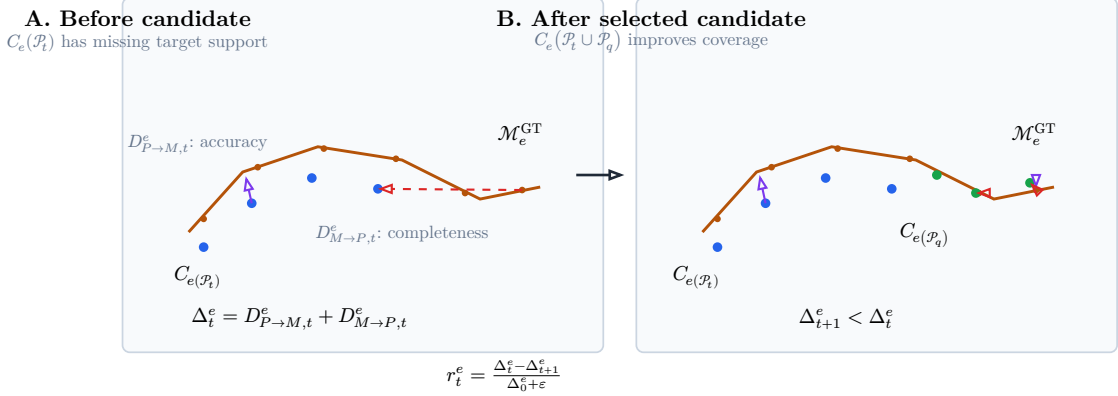
Figure 7: Target-specific point-mesh error behind RRI labels. Blue points are the target crop of accumulated oracle evaluation geometry, green points are the selected candidate contribution, the orange curve is the selected target mesh, purple witnesses indicate point-to-mesh accuracy, and dashed red witnesses indicate mesh-to-point completeness. Adding a valid candidate view is useful only insofar as it reduces the target-cropped aggregate error used by the oracle reward.
