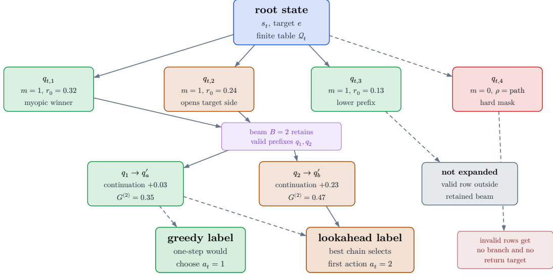
Figure 6: Bounded oracle-lookahead tree used as a rollout reference. Valid first-action rows may be expanded into selected-depth successor states and scored by cumulative root-normalized return G_t^{(H)} invalid rows are hard-masked and receive no branch. The selected first action can differ from the one-step greedy winner when a lower immediate reward opens a better second-step target view.
