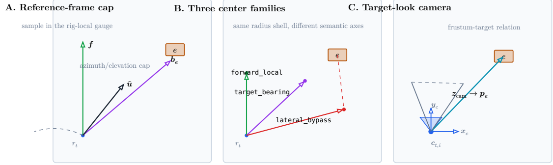
Figure 4: Schematic geometry of the core target-conditioned candidate families. The reference-frame direction support is reinterpreted as forward, target-bearing, or lateral-bypass motion, and target-looking cameras point toward the supplied target instruction. The manifest supplies family counts and all quantitative bounds.
