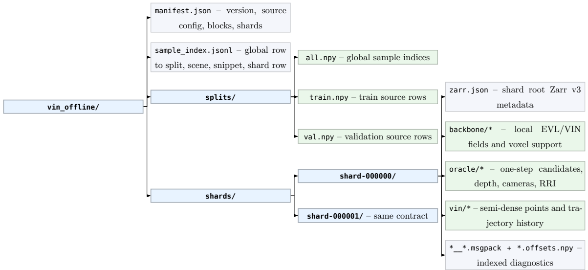
Figure 8: Immutable VIN offline-store schema. Row-aligned Zarr arrays store tensor fields, while indexed MessagePack blocks retain variable diagnostics. The main text needs the row roles and actor/oracle boundary; version-specific layout belongs in the resolved reproducibility record.
