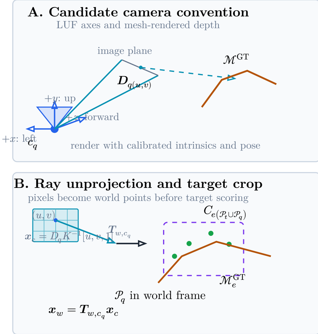
Figure 2: Camera-frame and ray contract behind oracle labels. Panel A fixes the candidate camera as a calibrated left-up-forward camera and renders depth from the GT mesh. Panel B shows the induced unprojection: a depth pixel becomes a camera-frame ray sample, is transformed into the world frame, enters the selected candidate point set, and is cropped against the selected target surface before target-specific error is scored [Met25a, Met25b].
