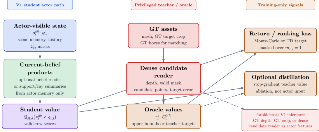
Figure 11: Teacher/student render path for leakage-safe training. The student branch consumes actor-visible state and current-belief render products, while privileged GT meshes, target crops, and dense candidate renders may produce oracle returns, teacher values, or distillation targets only. Dense GT candidate depth is therefore label or teacher evidence, not a V1 actor input.
