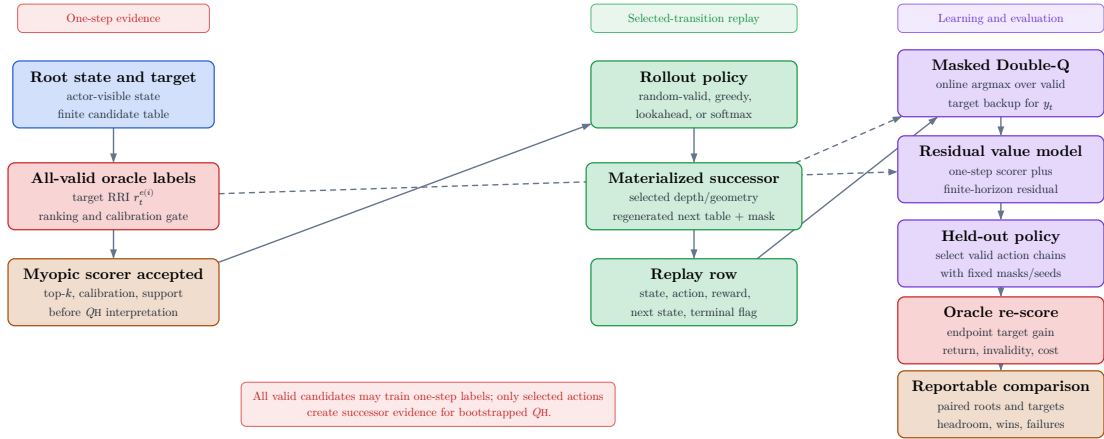
Figure 12: Selected-transition replay contract for Q_H . All valid candidates can receive one-step oracle target labels, but bootstrapped finite-horizon targets require materialized selected actions, successor counterfactual state, regenerated successor candidate tables, masks, terminal flags, and masked Double-Q targets.
