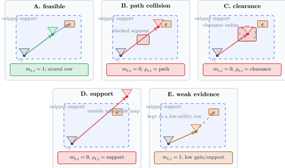
Figure 5: Candidate validity and pruning examples. The support envelope, mesh-clearance constraint, and path-collision check remove infeasible rows by setting m_{t,i} to false and recording an invalid-reason code \rho_{t,i} . A candidate with low target support or low expected gain remains valid if it satisfies the feasibility rules; it is a supervised low-utility row rather than an invalid action.
