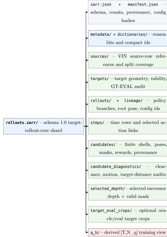
Figure 10: Implemented rollout replay schema. Row tables are the facts; q_h is a dense training cache validated against steps, candidates, retained chains, and targets.
