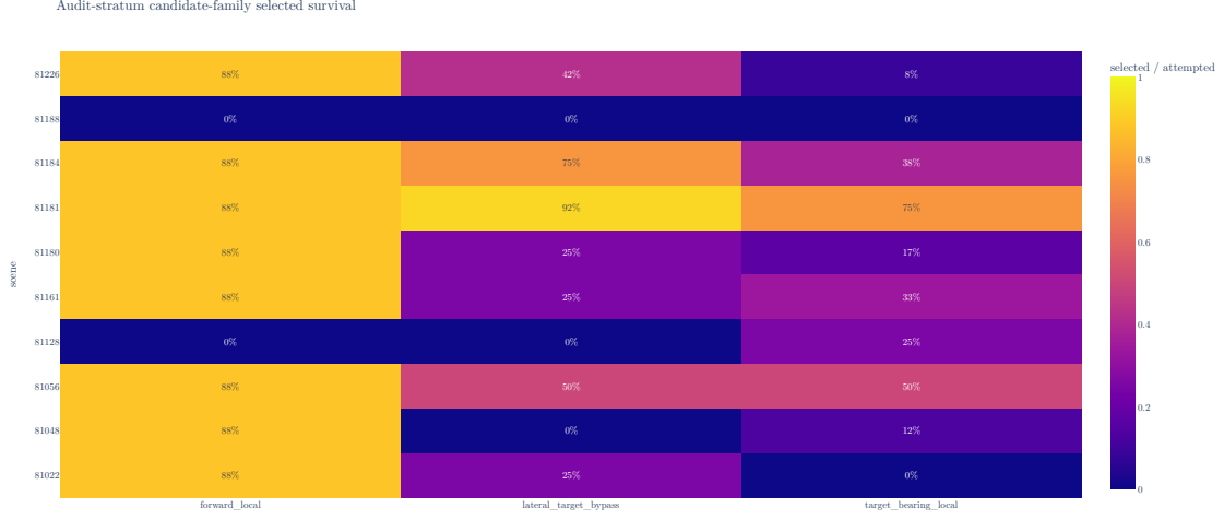
Figure 11: Candidate-family survival for one deterministic scene from each of the ten persisted Phase-A audit strata. Each cell reports compact-valid-shell membership divided by attempted rows for one factual state and proposal family. The complete 100-state matrix remains in the evidence bundle. The artifact is bound to clean execution revision 2baf7cf6b276b81c50d01d45b152016d7cf68033 , generation revision a2ae86b7463930c9 , and artifact SHA-256 6c7fa8cb249687b80867261db1d1c7d1906e6b01f54d3cca3db4bfcba7bc670 . The stored shells and execution identity are unchanged; provenance correction revision phase-a-path-independent-config-reseal-v1 replaces checkout-dependent configuration paths with the separately verified source store identity.
