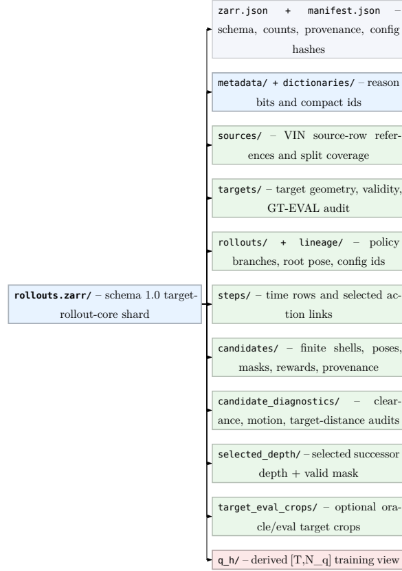
Figure 11: Implemented standalone rollout replay schema. The row tables are the canonical facts; q_h/ is a persisted cache for high-throughput finite-candidate training and is validated against steps/ , candidates/ , rollouts/ , and targets/ .
