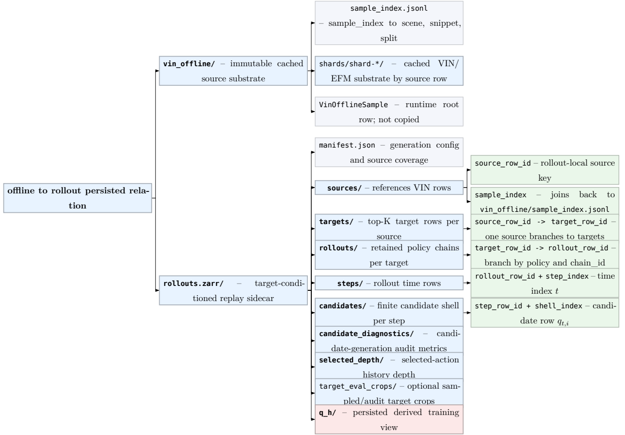
Figure 10: Persistent relation between immutable VIN offline rows and target-conditioned rollout rows. rollouts.zarr/ stores joins, target tasks, selected branches, candidate masks, selected-depth successor history, and a derived Q_H training view; it does not copy or rewrite the heavy source substrate.
