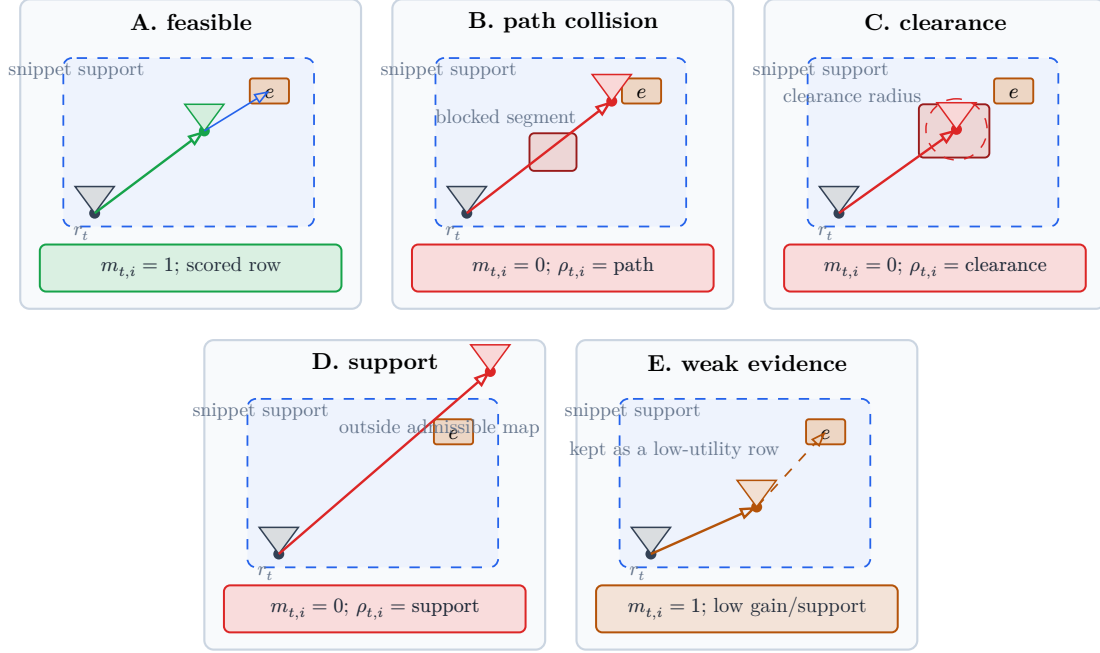
Figure 6: Candidate validity and pruning examples. The support envelope, mesh-clearance constraint, and path-collision check remove infeasible rows by setting m_{t,i} to false and recording an invalid-reason code \rho_{t,i} . A candidate with low target support or low expected gain remains valid if it satisfies the feasibility rules; it is a supervised low-utility row rather than an invalid action.
