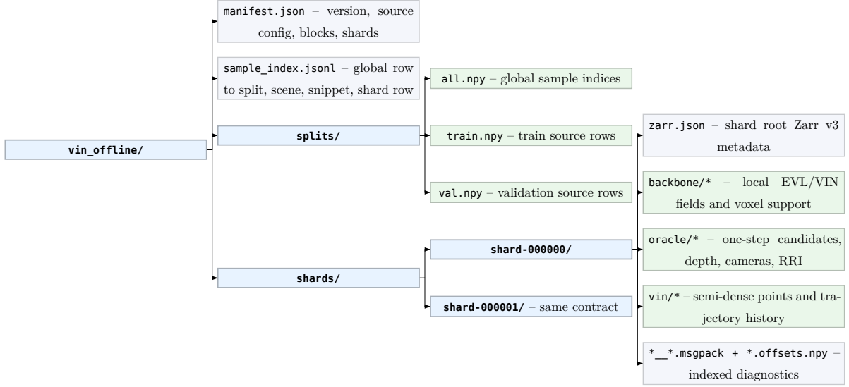
Figure 9: Immutable VIN offline-store schema. The live v7 store writes row-aligned Zarr arrays directly inside each shard group and uses indexed MessagePack record blocks for variable diagnostics. The thesis needs the row-level roles and actor/oracle boundary; chunking and byte-level layout belong in reproducibility notes.
