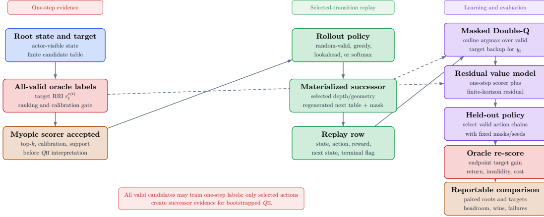
Figure 18: Selected-transition replay contract for Q_H . All valid candidates can receive one-step oracle target labels, but bootstrapped finite-horizon targets require materialized selected actions, successor counterfactual state, regenerated successor candidate tables, masks, terminal flags, and masked Double-Q targets.
