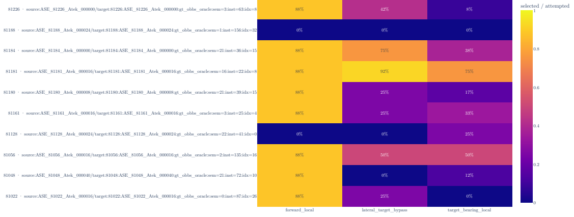
Figure 11: Candidate-family survival for one deterministic scene from each of the ten persisted Phase-A audit strata. Each cell reports compact-valid-shell membership divided by attempted rows for one factual state and proposal family. The complete 100-state matrix remains in the evidence bundle. The artifact is bound to clean execution revision 2baf7cf6b276b81c50d01d45b152016d7cf68033 , generation revision a2ae86b7463930c9 , and artifact SHA-256 6d33e9e3d68737c8a6a5589ae5117c1e4d7fcaa89056fcfcaec1d315e4509c83 . The stored shells, support counts, verdict, and execution identity are unchanged. Geometry correction revision phase-a-target-aligned-z-up-v1 rotates the authenticated candidate centres, target-relative vectors, and view directions into the canonical target-aligned world-Z-up basis without rerunning candidate generation. Its predecessor artifact is 60b271db515a5e665fcb7bbeecb87e6acb4bac2ff8e28b26b7308911328759c .
