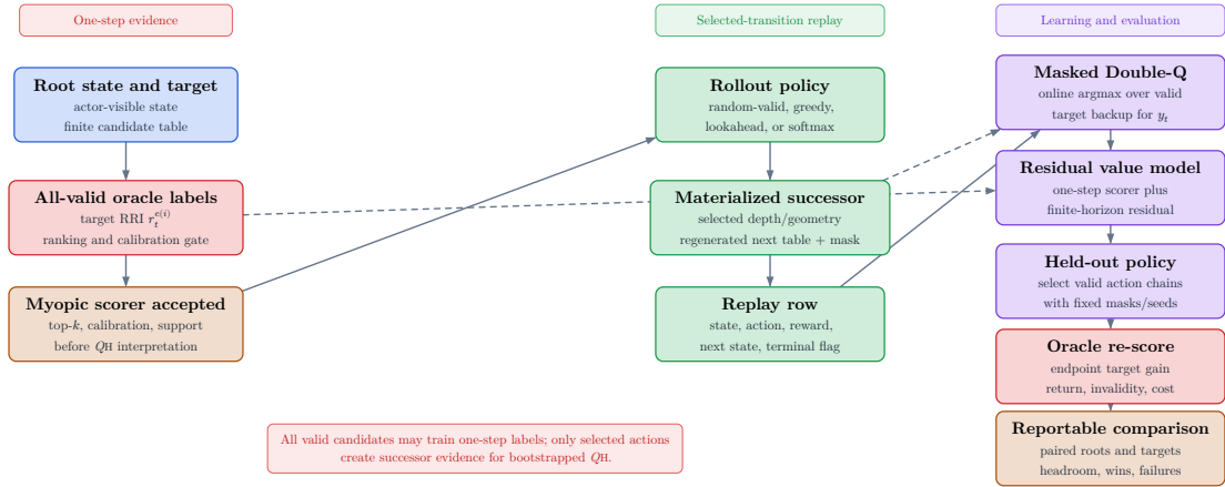
Figure 10: Selected-transition replay contract for Q_H . All valid candidates can receive one-step oracle target labels, but bootstrapped finite-horizon targets require materialized selected actions, successor counterfactual state, regenerated successor candidate tables, masks, terminal flags, and masked Double-Q targets.
