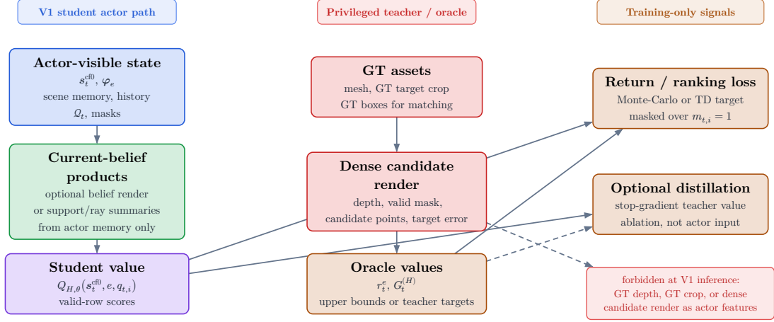
Figure 9: Teacher/student render path for leakage-safe training. The student branch consumes actor-visible state and current-belief render products, while privileged GT meshes, target crops, and dense candidate renders may produce oracle returns, teacher values, or distillation targets only. Dense GT candidate depth is therefore label or teacher evidence, not a V1 actor input.
