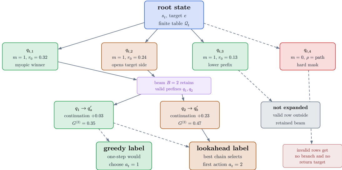
Figure 4: Bounded oracle-lookahead tree used as a rollout reference. Valid first-action rows may be expanded into selected-depth successor states and scored by cumulative root-normalized return G_t^{(H)} invalid rows are hard-masked and receive no branch. The selected first action can differ from the one-step greedy winner when a lower immediate reward opens a better second-step target view.
