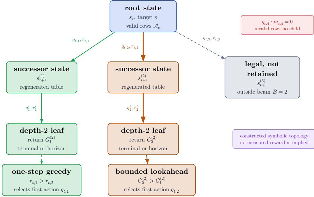
Figure 5: Constructed symbolic topology of the bounded oracle-lookahead reference. Nodes are counterfactual states and edge labels are candidate actions with immediate rewards. Only valid first-action rows produce children; the beam retains a bounded prefix set, and invalid rows receive no branch. The inequalities illustrate how the selected first action can differ from one-step greedy without inventing measured reward values.
