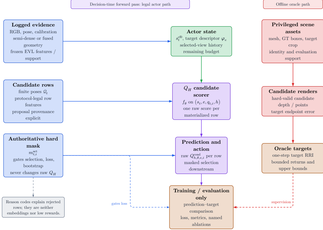
Figure 1: Actor and oracle boundary. Logged evidence, target context, and protocol-legal candidate features feed the mask-independent Q_H scorer. The authoritative hard mask instead gates selection, supervised rows, and bootstrap support. GT assets generate renders and oracle targets that meet predictions only after the forward pass, in loss and metrics. Reason codes remain audit evidence rather than embeddings or low rewards.
