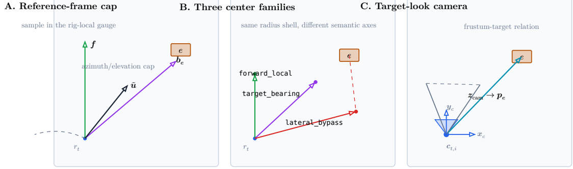
Figure 5: Schematic geometry of the target-conditioned three-family candidate shell. Panel A shows the root/reference-frame direction cap; panel B shows how the same shell support is reinterpreted by the forward-local, target-bearing, and lateral-bypass center families; panel C shows the target-look camera construction and the resulting target-frustum relation. Exact sampling densities, radius draws, and pruning constraints are defined by the surrounding equations, not by the schematic scale.
