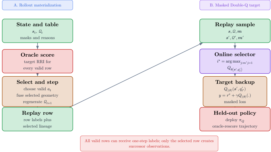
Figure 12: Replay-to-learning process for finite-candidate Q_H . Panel A separates all-valid-row oracle labels from the one selected action that materializes successor geometry and a regenerated candidate table. Panel B shows the masked Double-Q backup: the online network selects a valid successor row, the target network evaluates that row, and held-out policy quality is measured only by oracle re-scoring selected trajectories [HGS15].
