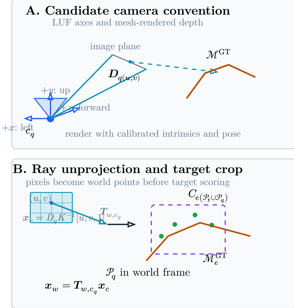
Figure 3: Camera-frame and ray contract behind oracle labels. Panel A fixes the candidate camera as a calibrated left-up-forward camera and renders depth from the GT mesh. Panel B shows the induced unprojection: a depth pixel becomes a camera-frame ray sample, is transformed into the world frame, enters the selected candidate point set, and is cropped against the matched target surface before target-specific error is scored [Met25a, Met25c].
