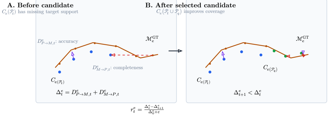
Figure 6: Target-specific point-mesh error behind RRI labels. Blue points are the target crop of accumulated actor-visible geometry, green points are the selected candidate contribution, the orange curve is the matched target mesh, purple witnesses indicate point-to-mesh accuracy, and dashed red witnesses indicate mesh-to-point completeness. Adding a valid candidate view is useful only insofar as it reduces the target-cropped aggregate error used by the oracle reward.
