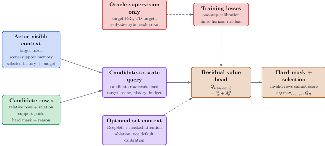
Figure 14: Default candidate-query Q_H architecture contract. Actor-visible target, scene, history, budget, candidate self/relation, mask, and provenance descriptors feed a candidate-to-state query encoder; the residual value head decodes finite-horizon values only for hard-valid rows, while oracle target RRI, TD targets, and endpoint metrics supervise losses and evaluation outside the actor-input graph. Optional set context is an ablation rather than the default source of absolute value calibration.
