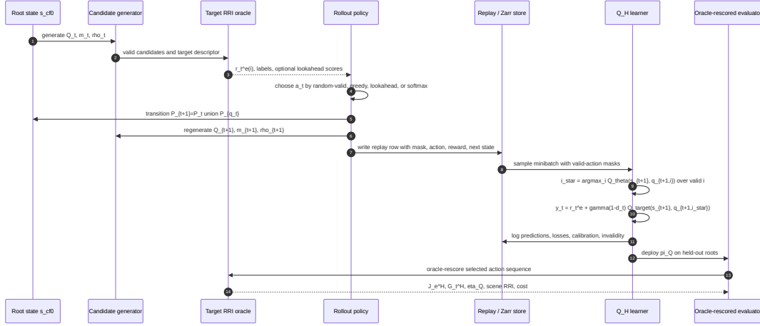
Figure 16: Selected-transition replay contract for Q_H . All valid candidates can receive one-step oracle target labels, but bootstrapped finite-horizon targets require materialized selected actions, successor counterfactual state, regenerated successor candidate tables, masks, terminal flags, and masked Double-Q targets.
