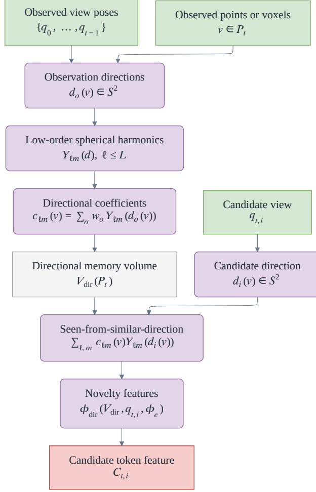
Figure 11: Actor-visible directional memory for target-local view novelty. The figure shows a planned descriptor branch, not an implemented performance result: selected view directions over observed points or voxels are summarized as low-order directional coefficients or second moments, and each valid candidate reads the memory to produce a candidate token feature for Q_H .
