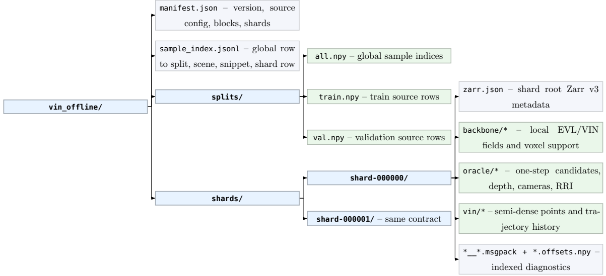
Figure 7: Immutable VIN offline-store schema. The live v7 store writes row-aligned Zarr arrays directly inside each shard group and uses indexed MessagePack record blocks for variable diagnostics. The thesis needs the row-level roles and actor/oracle boundary; chunking and byte-level layout belong in reproducibility notes.
