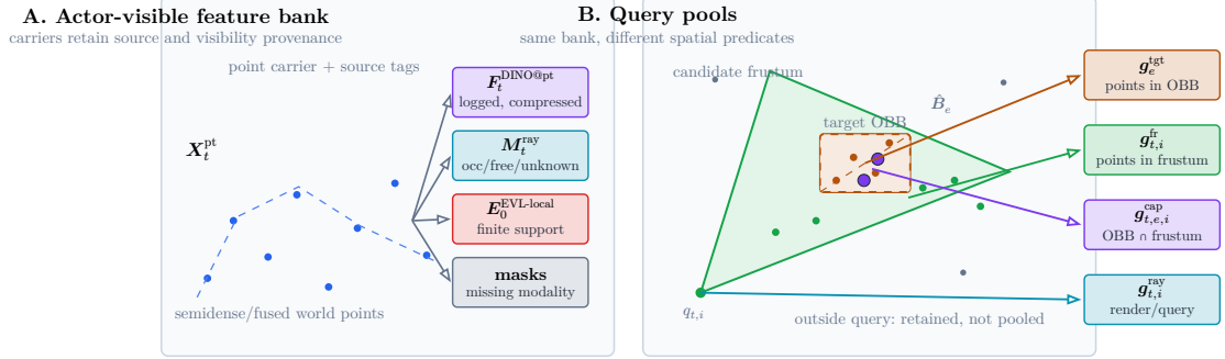
Figure 10: Actor-visible feature-bank query pools for Q_H . Panel A separates point carriers, optional logged DINO descriptors, ray-memory evidence, root-local EVL support, and missing-modality masks. Panel B shows that the target pool, candidate-frustum pool, target-frustum-intersection pool, and ray query are different spatial predicates over the same actor-visible memory, not fresh counterfactual visual observations.
