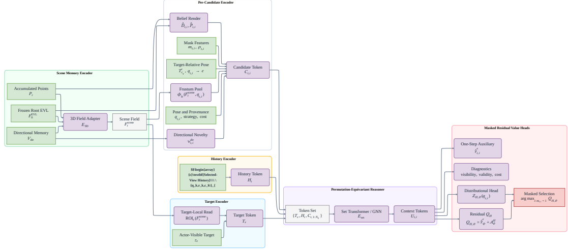
Figure 6: Candidate-query Q_H architecture sketch. Actor-visible EVL evidence, accumulated geometry, target descriptors, selected-history summaries, candidate geometry, masks, and directional memory feed a permutation-equivariant set reasoner; residual finite-horizon values, one-step auxiliary scores, and diagnostics are then decoded only over valid candidate rows. Oracle labels supervise training and evaluation outside this actor-input graph.
