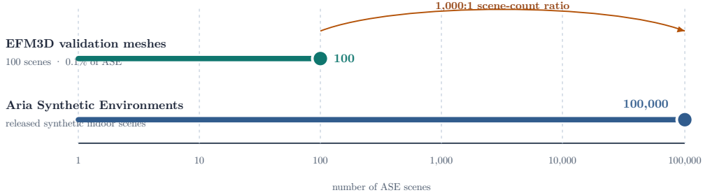
Figure 2: Scale of the released ASE corpus and the EFM3D ground-truth-mesh evaluation subset. A logarithmic scene-count axis locates 100 mesh validation scenes against 100,000 ASE scenes; the subset is 0.1% of the corpus (a 1,000:1 ratio). This schematic quantitative comparison is derived from the cited release counts. [Met25a, Str+24a]
