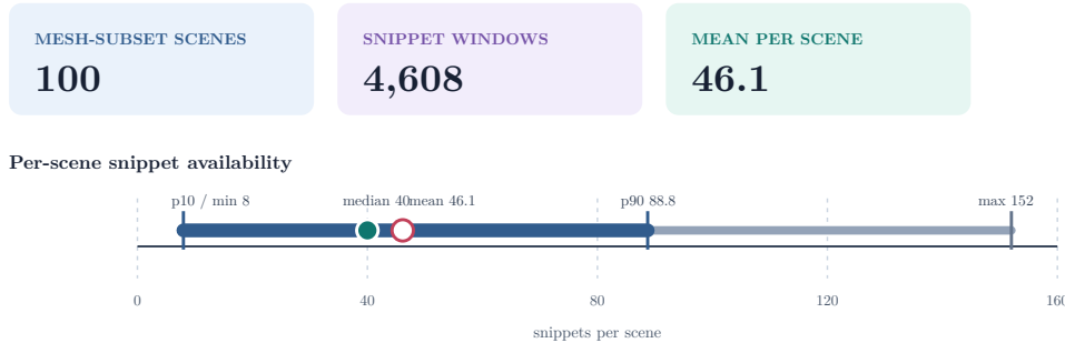
Figure 3: Fresh summary of per-scene availability in the locally scanned ATEK–EFM snapshot (scan date: 2025-12-31). The range, percentile interval, median, and mean characterize 4,608 windows across 100 scenes. This data-derived figure scopes local experimental availability, not the global ASE distribution.
