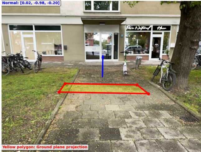
(a) RANSAC ground plane detection for height estimation.
