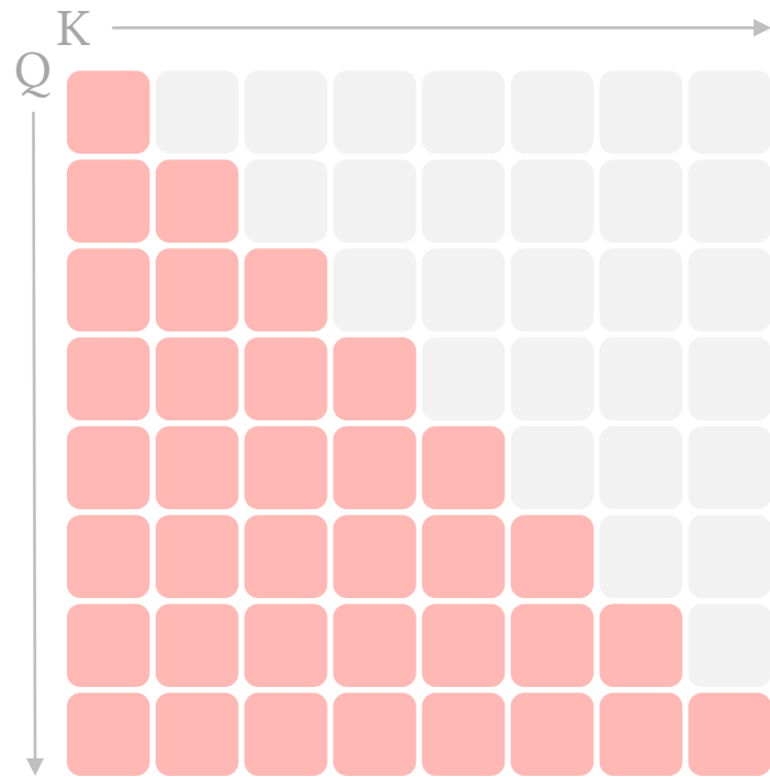
Causal Attention (b)
