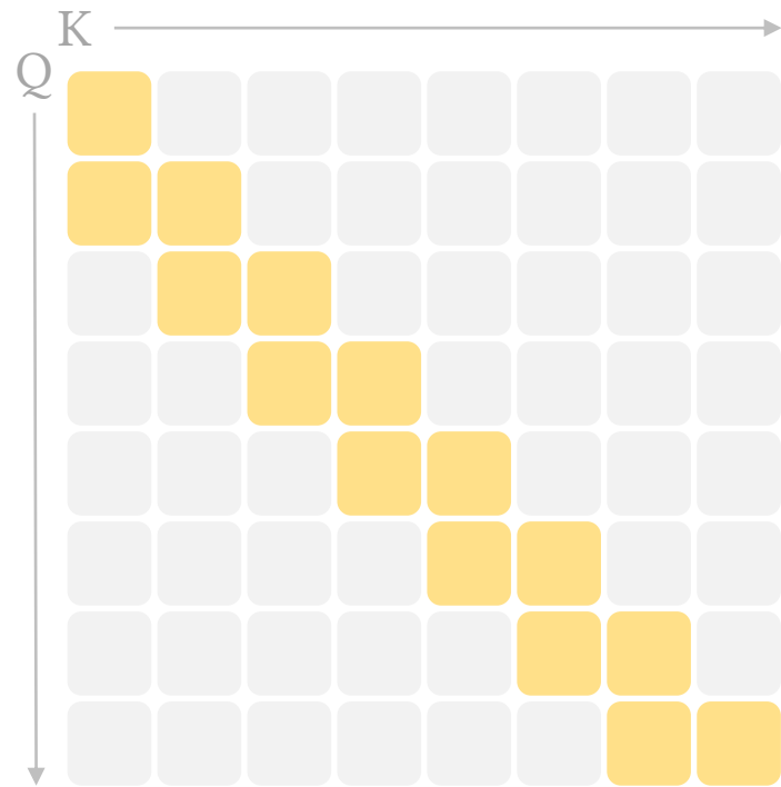
Sliding Window Attention (c)
