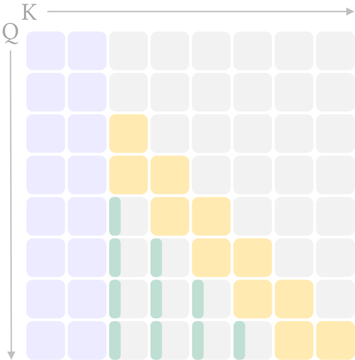
Geometric Context Attention
