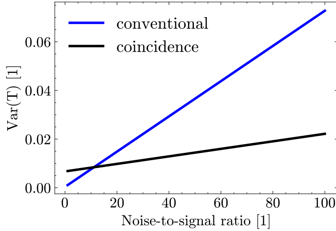
Figure 13.: Variance of the transmittance as a function of the noise-to-signal ratio
