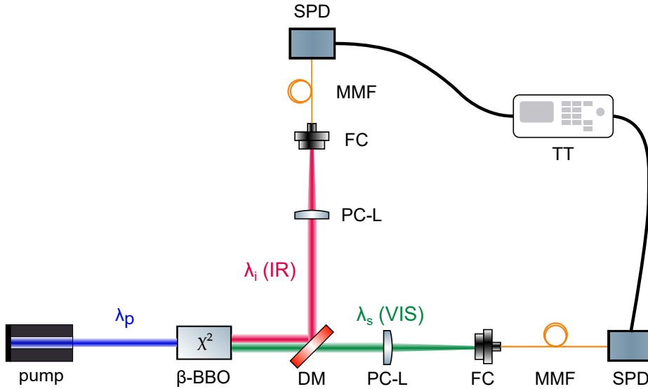
Figure 3.: Simplified sketch of the experimental setup; DM: dichroic mirror, FC: fiber coupling, MMF: multi-mode fiber, PC-L: plano-convex lens, Sam: sample, SPD: single photon detector, TT: time tagging unit
