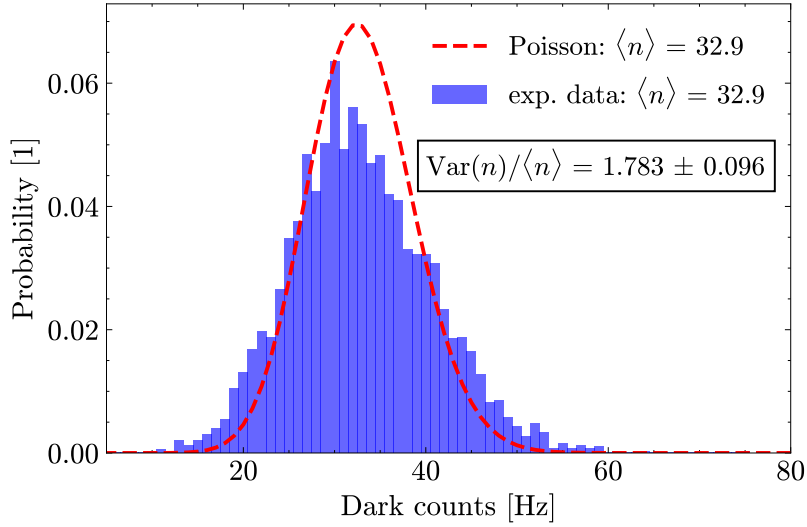
Figure 6.: Dark counts of the IR single photon detector in the idler arm
