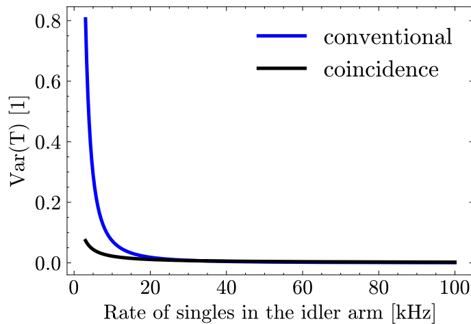
Figure 16.: Variance of the transmittance as a function of the photon rate in the idler arm
