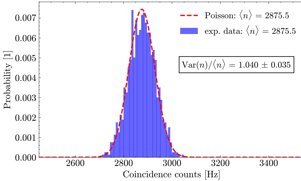
Figure 10.: Photon statistics of the coincidence counts
