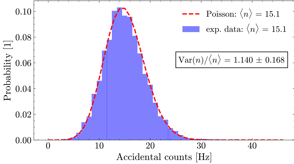
Figure 11.: Photon statistics of the accidental counts
