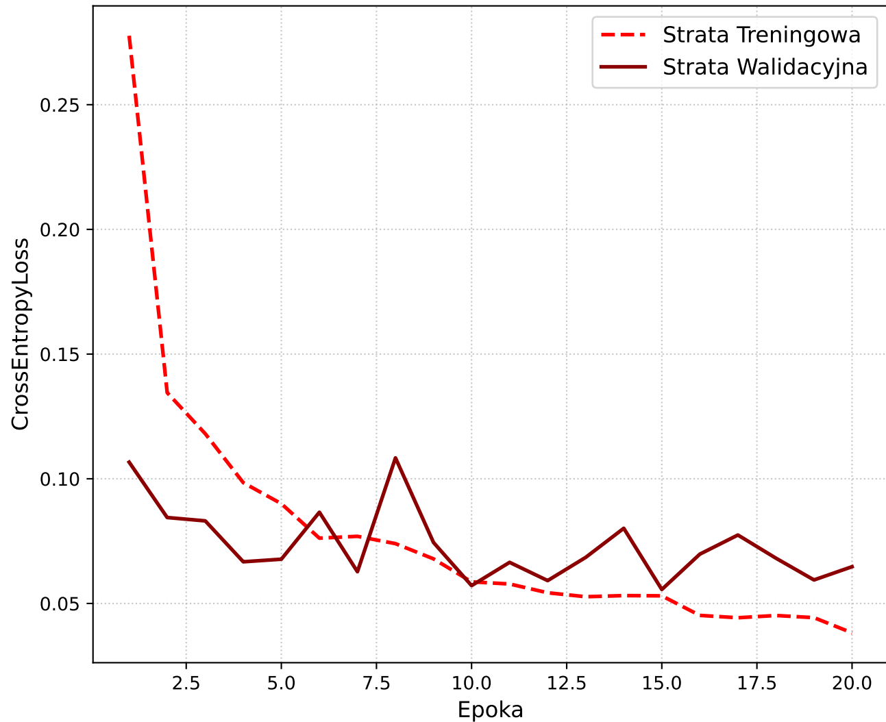
Loss
