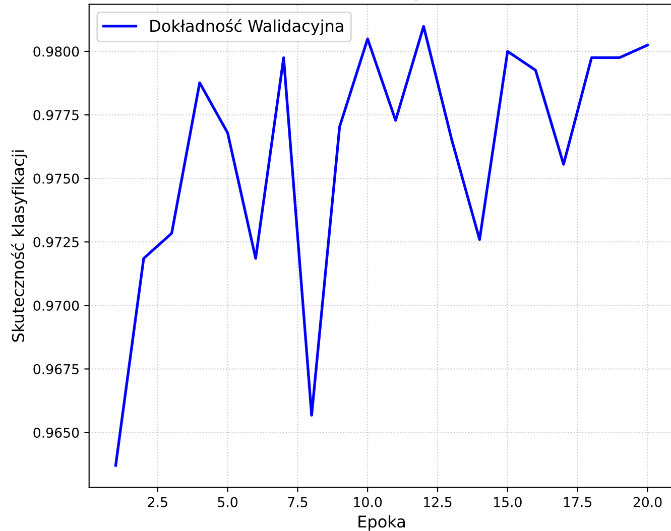
Accuracy
