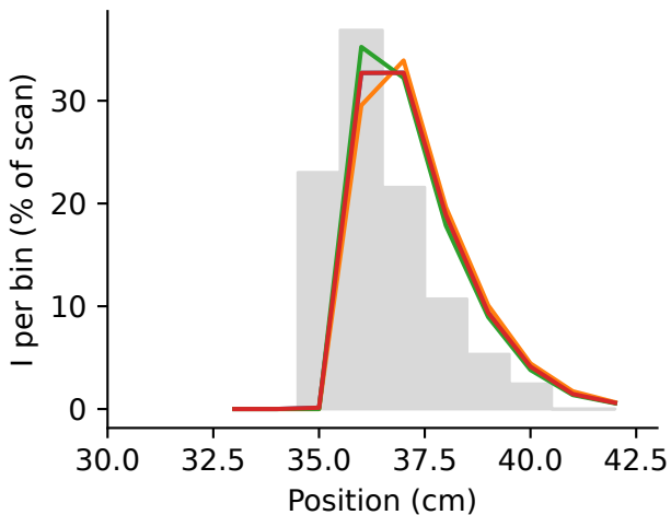
Steel Q2, 1%
