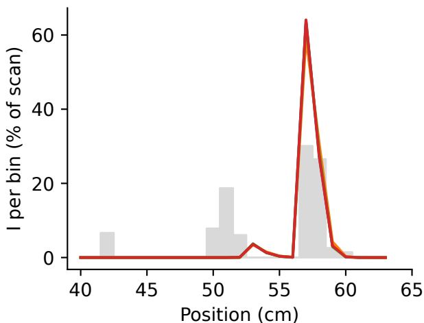
Steel Q2, 1%
